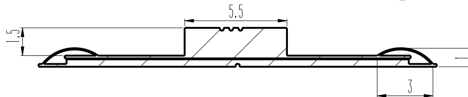
SECTION B-B SCALE 5.000
