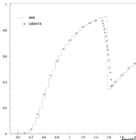
Figure 2: Simulation of photon transmission in 1\mu\text{m} Al layer, showing the evidence of shell effects; the solid line represents experimental data from [4] the dots are the simulation results with Geant4 Low Energy Electromagnetic package.
