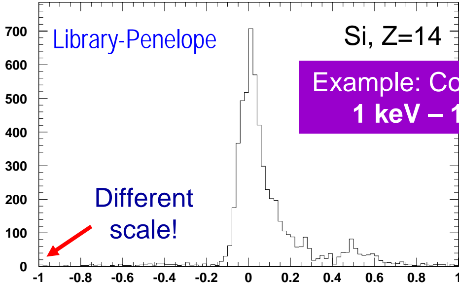
Compton cross section (Library-Penelope)%
