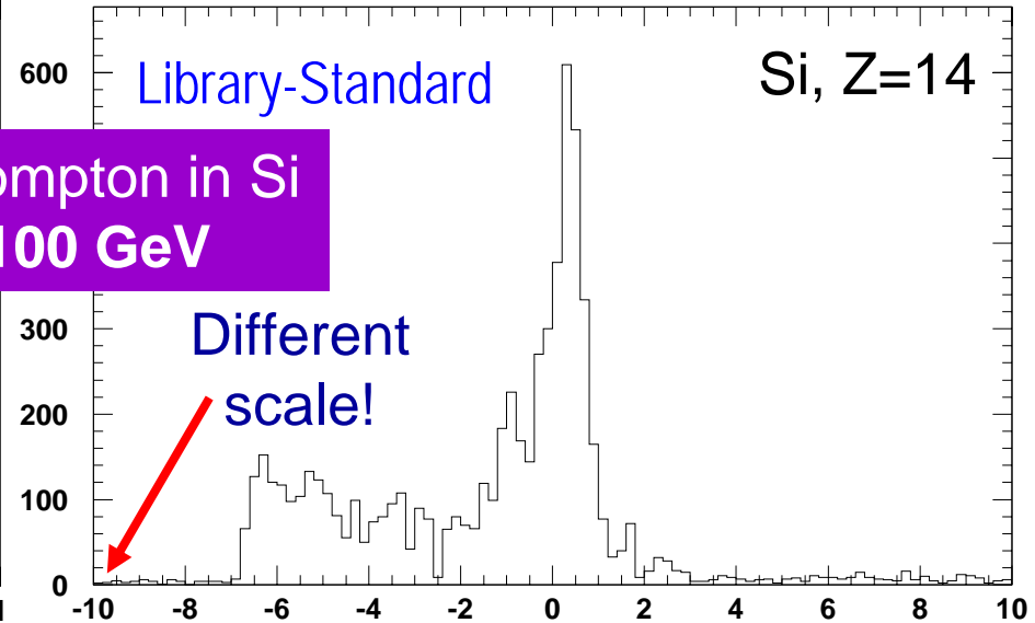
Compton cross section (Library-Standard)%
