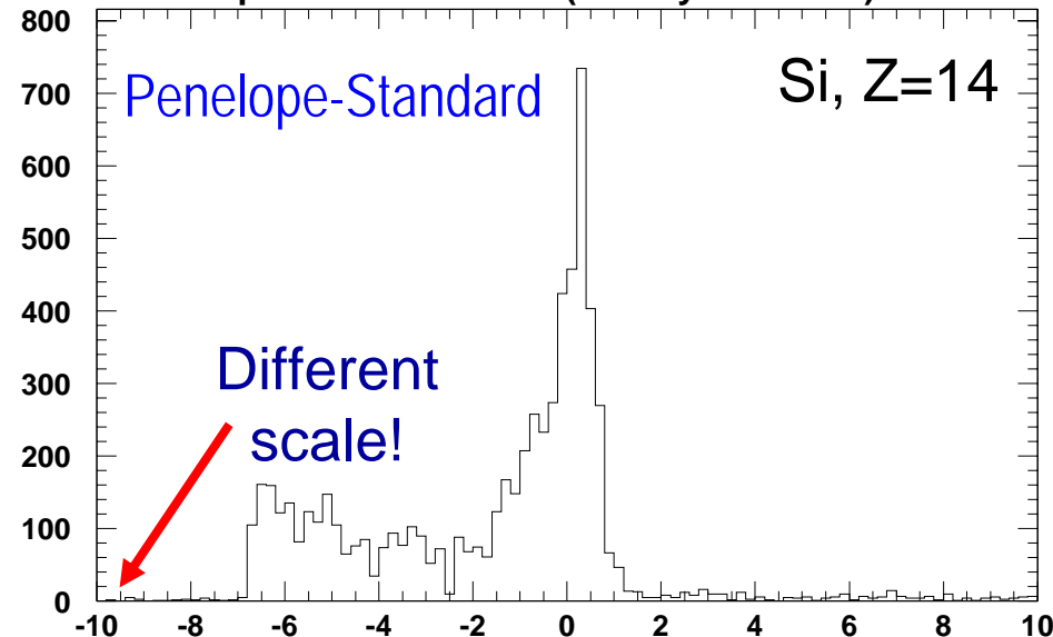
Compton cross section (Penelope-Standard)%
