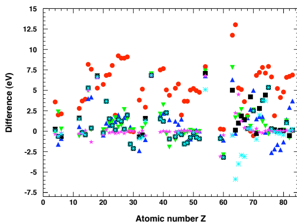
Median relative intensity deviation per isotope for X-ray emission
