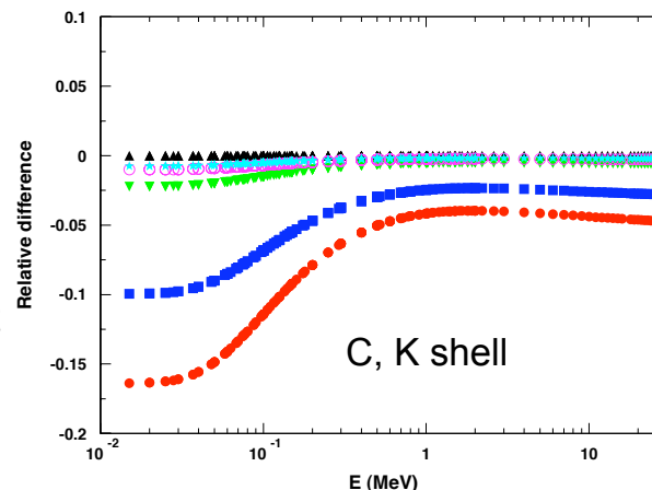
Proton ionisation cross section using different atomic data, compared to measurements
