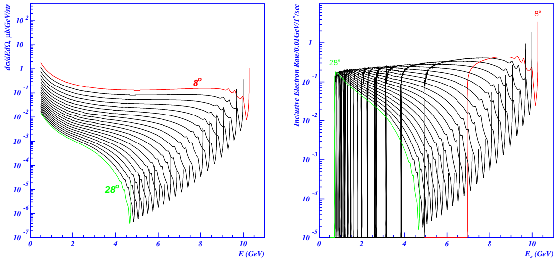
Figure 16: Cross sections (left) and rates at 10^{35} \text{ cm}^{-2} \text{ sec}^{-1} (right) for inclusive electron scattering, ep \rightarrow e'X , at 11.5 GeV as a function of scattered electron energy, for scattered angles from 8^\circ to 28^\circ . Calculations done using the code of Ref. [80].
