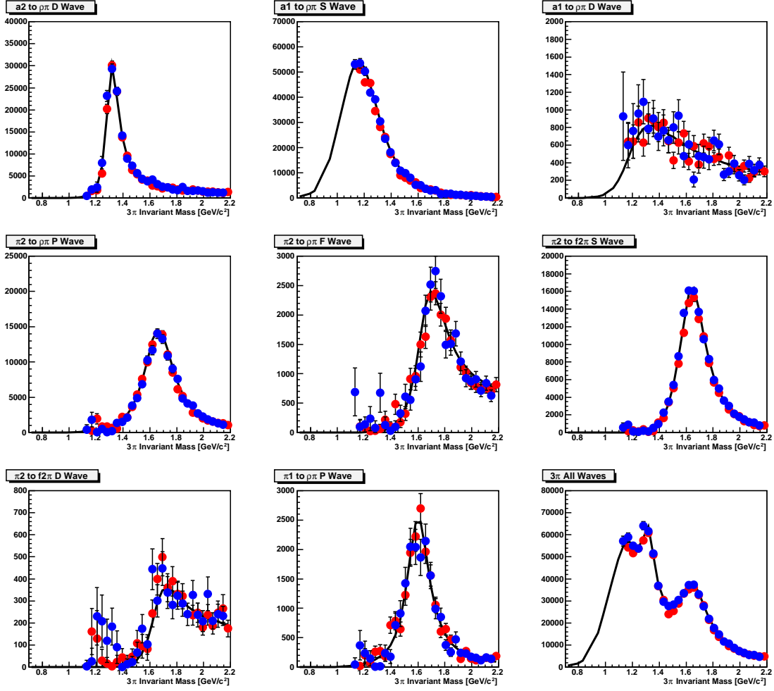
Figure 30: The intensities of the 8 different isobar channels in the 3\pi model, see table 5. The bottom right plot shows the total intensity. The black line shows the generated waves, while the blue and red points are the fit results for t = 0.2 and 0.5(GeV/c)^2 , respectively.
