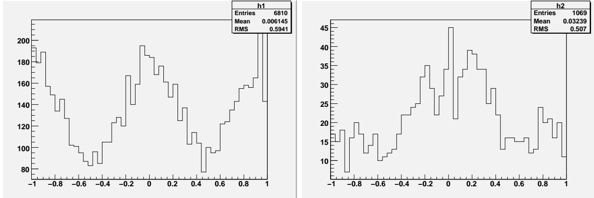
Figure 28: The raw (left) and accepted (right) \phi_{GJ} distributions for the \eta\pi final state.
