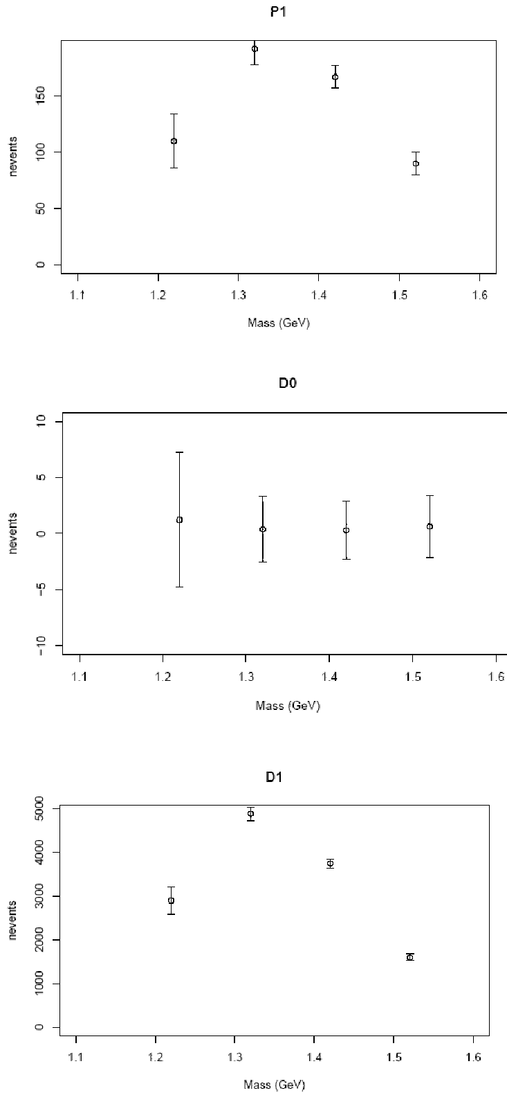
Figure 29: The PWA intensities resulting from the mass independent PWA fits of the simulated data. One expects not to observe resonance structure in these partial waves.
