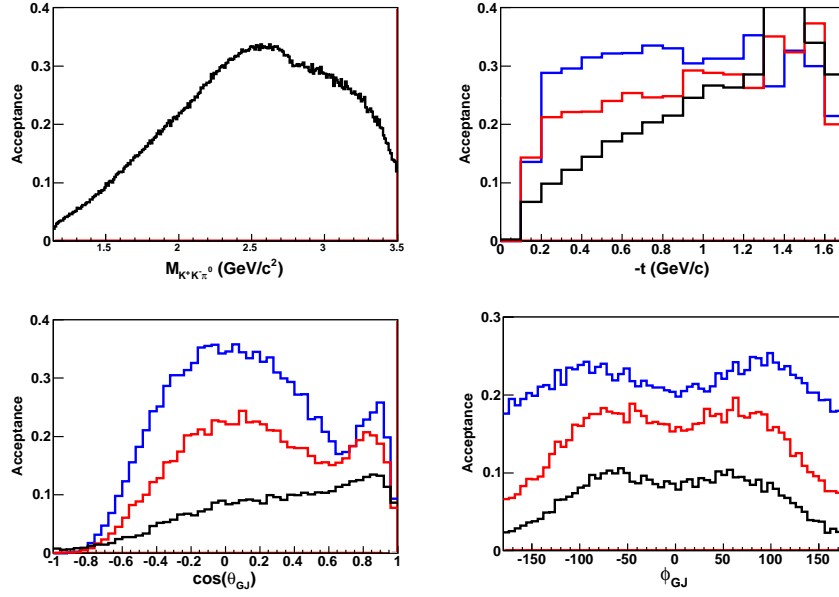
Figure 25: Acceptances for the K^+K^-\pi^0p final state, with the K^- reconstructed. Top left the K^+K^-\pi^0 invariant mass M_{K^+K^-\pi^0} , right the momentum transfer t , bottom left, \cos\theta_{GJ} and right, \phi_{GJ} . For the latter 3 plots the black, red and blue lines correspond to M_{K^+K^-\pi^0} = 1.4, 1.7 and 2.0 ( \text{GeV}/c^2 ) respectively.
