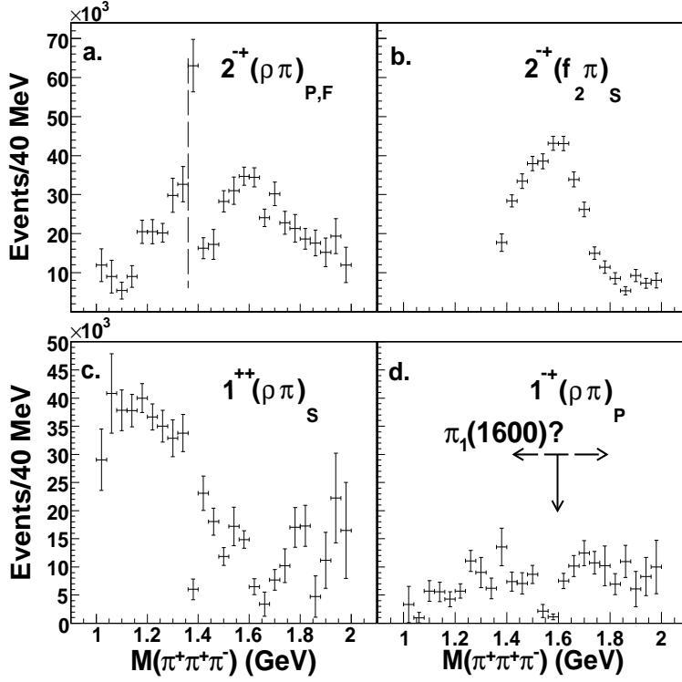
Figure 4: CLAS PWA results on 3\pi photoproduction [17].
