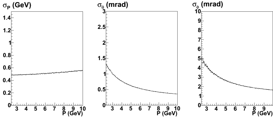
Figure 19: FASTMC resolutions for e^- at \theta = 15^\circ . The curves are based on GEANT4 simulation of the CLAS12 tracking system and reconstruction by the SOCRAT package [84, 70].
