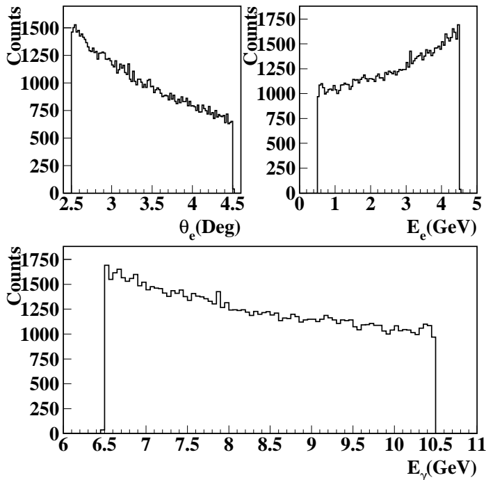
Figure 7: Angular and energy distribution of scattered electrons (top) and virtual photon energy distribution (bottom) within the geometrical and momentum acceptance of the FT.
