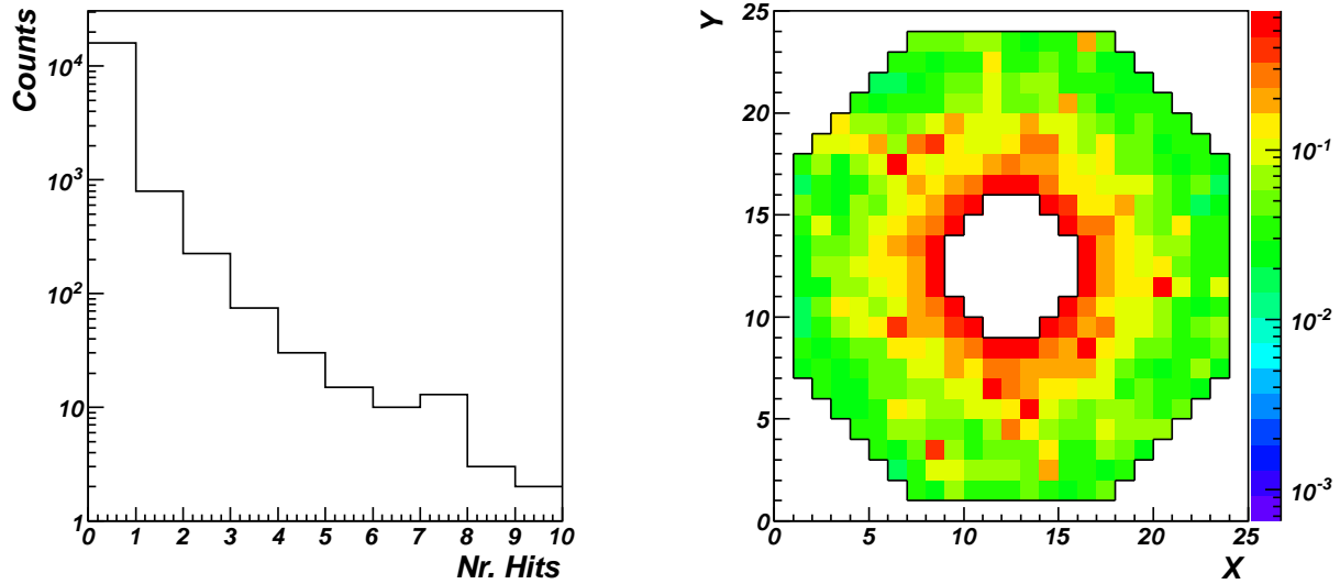
Figure 13: Left: number of crystals in the FT calorimeter with signal above threshold in a 20 ns time window due to the electromagnetic background at a luminosity of 10^{35} \text{ cm}^{-2}\text{s}^{-1} . Right: distribution of the energy deposited in the calorimeter in a 20 ns window; the z-scale is in MeV.
