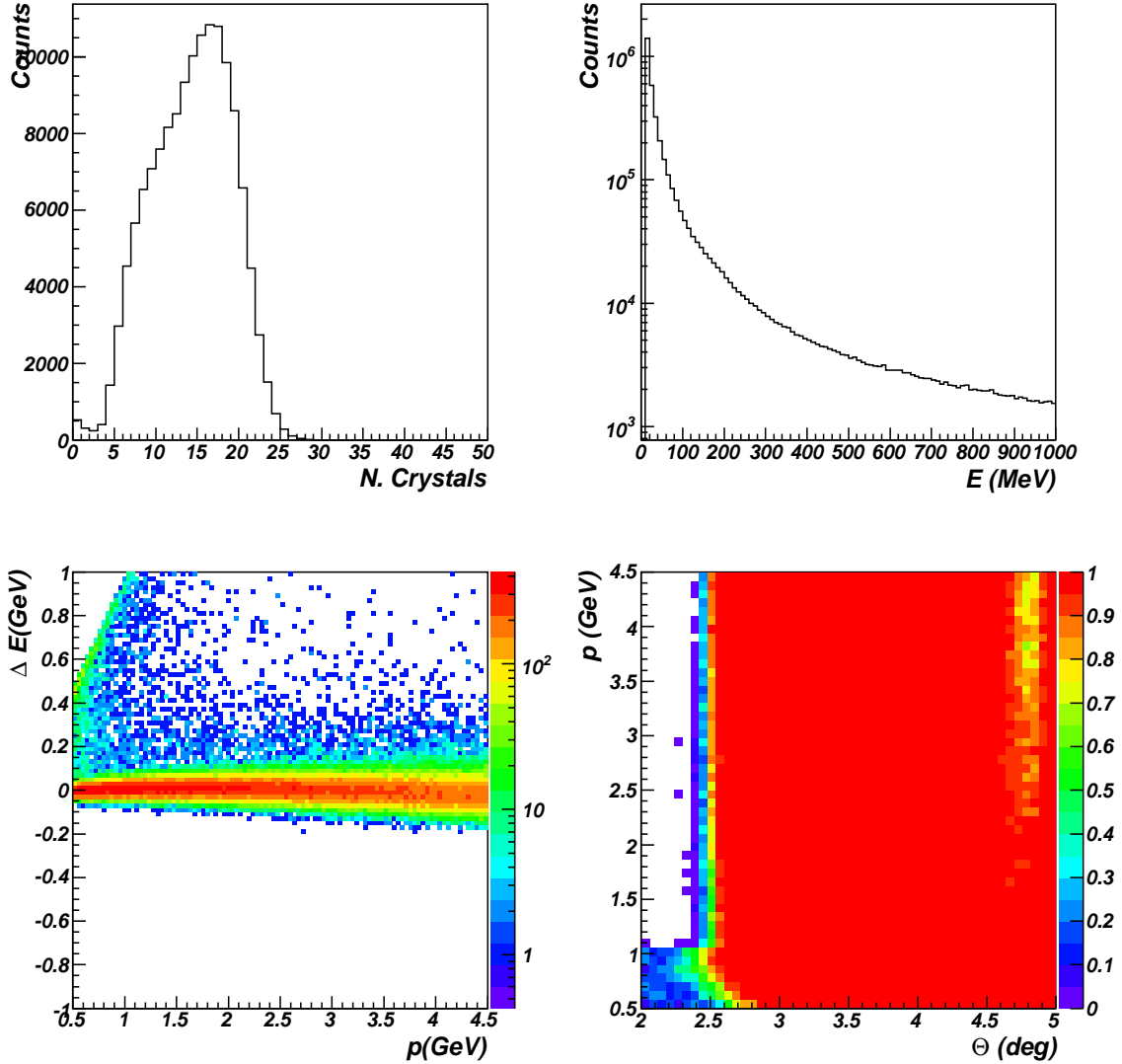
Figure 11: GEMC simulation results. Top-left: Number of crystals with deposited energy greater than 10 MeV involved in the cluster generated by an incoming electron with energy of 0.5-4.5 GeV. Top-right: energy deposited in a single crystal. Bottom-left: difference between the reconstructed and generated electron energy as a function of the electron momentum. Bottom-right: ratio between detected over generated electrons in the kinematic of interest. All plots are based on simulations of electrons generated uniformly in the momentum range 0.05-5 GeV and polar angle range 1^\circ - 35^\circ .
