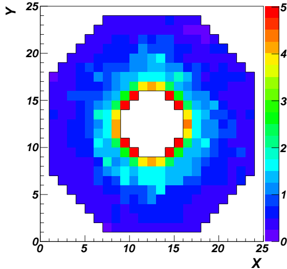
Figure 14: Radiation dose on the FT calorimeter crystals in rad/hour at 10^{35} \text{ cm}^{-2}\text{s}^{-1} luminosity. The maximum values of about 5 rad/h are observed for the innermost crystals, i.e. at the smaller angles.
