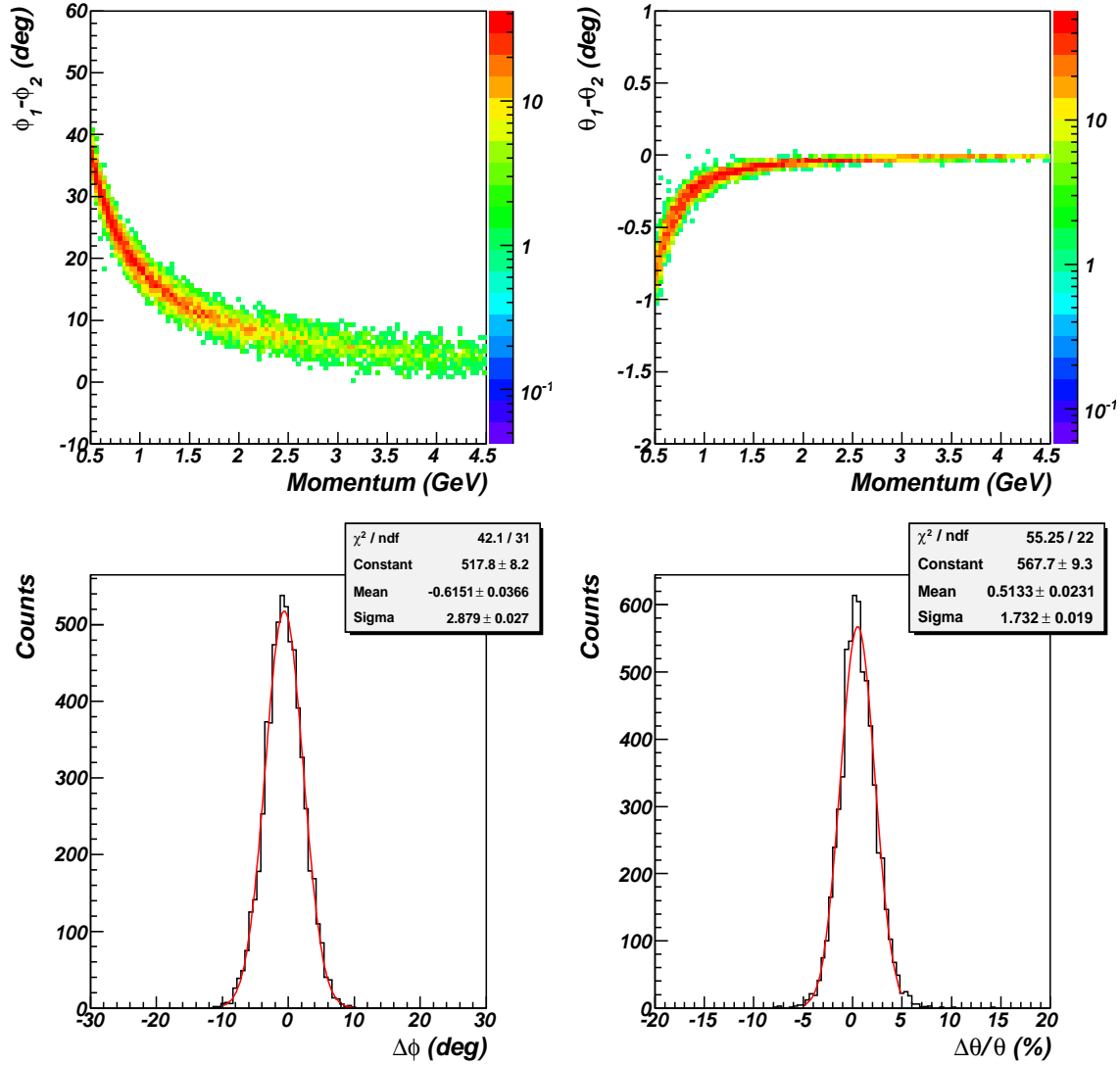
Figure 10: GEMC simulation results. Top: difference between the azimuthal and polar angles measured at two tracking planes as a function of the particle momentum. Bottom: resolution on the reconstruction of the particle vertex angles estimated from the simulation assuming 200 \mu\text{m} spatial resolution of the tracker and the presence of air in between the tracking planes.
