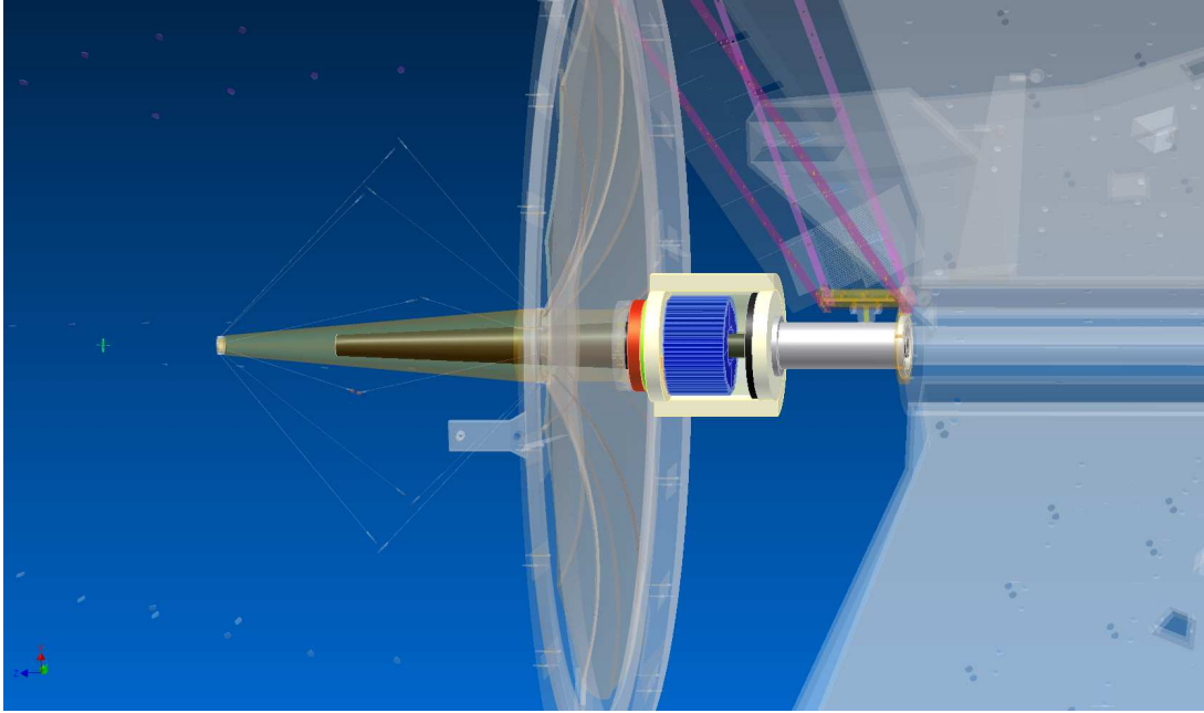
Figure 6: CAD drawing showing the integration of the FT in CLAS12. The FT is located in the free space between the HTCC and the first DC layer. The FT calorimeter shown in blue is located at about 190 cm from the interaction point, shown by the green cross, and is enclosed in a Rohacell case to provide thermal insulation. The scintillation counter (green) and first tracker layer (red) are located in front of the calorimeter. A tungsten cone in black shield the FT from Møller electrons and electromagnetic background created by the beam.
