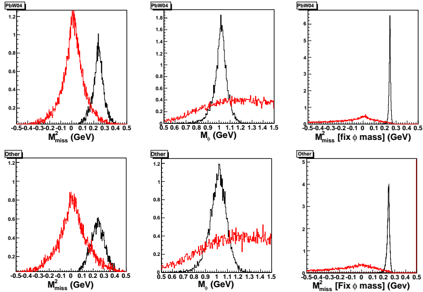
Figure 26: Reconstructed masses from the pK^+\gamma final state for the CLAS-IC tagger (top) and the lowest resolution tagger (bottom). In all plots, the black line shows the final state of interest, while the red line is for a phase space \gamma p \rightarrow K^+\pi^0\pi^-p reaction. The left plot shows the missing mass ( \sim K^- ), the middle the reconstructed \phi mass and the right plot the missing, mass having fixed the reconstructed \phi mass to 1.020 GeV.
