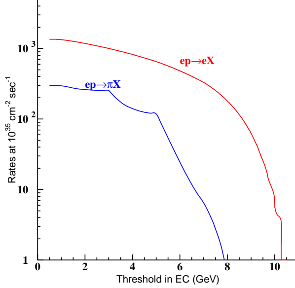
Figure 17: Trigger rates integrated over production angles as a function of the minimum energy (trigger threshold) for inclusive electron and \pi^{+/-} production at luminosity of 10^{35} \text{ cm}^{-2} \text{ sec}^{-1} . \pi^- yields from Ref. [81] were used to estimate pion rates, assuming the \pi^+ yield is twice the \pi^- yield. In the trigger, cuts on the number of photoelectrons in the HTCC and on deposited energy in the EC are used.
