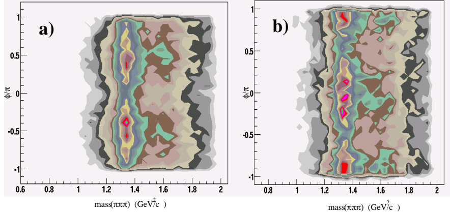
Figure 38: The \phi/\pi vs. \text{Mass}[3\pi] for those events with the polarization perpendicular to the production plane (left) and in the production plane (right). The simulated polarization was set to 60%.
