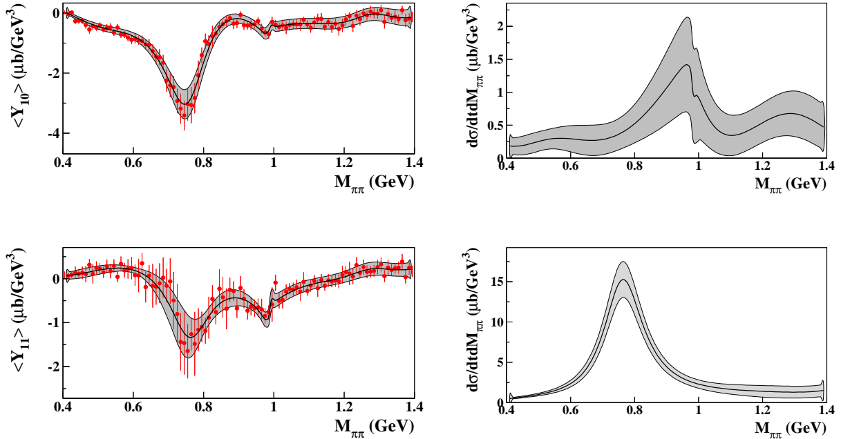
Figure 3: Left: Y_{10} , Y_{11} moments of the di-pion decay angular distribution in the photon energy range E_\gamma = 3.2 - 3.4 GeV and momentum transfer range -t = 0.5 - 0.6 GeV 2 as a function of the di-pion mass. Right: differential cross section associated to the S (top) and P (bottom) waves.
