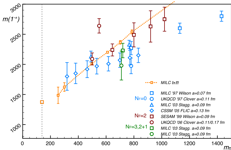
Figure 2: Summary of lattice results for the mass of the J^{PC} = 1^{-+} exotic meson. Data are from Refs. [11, 12, 13, 14, 15, 16].
