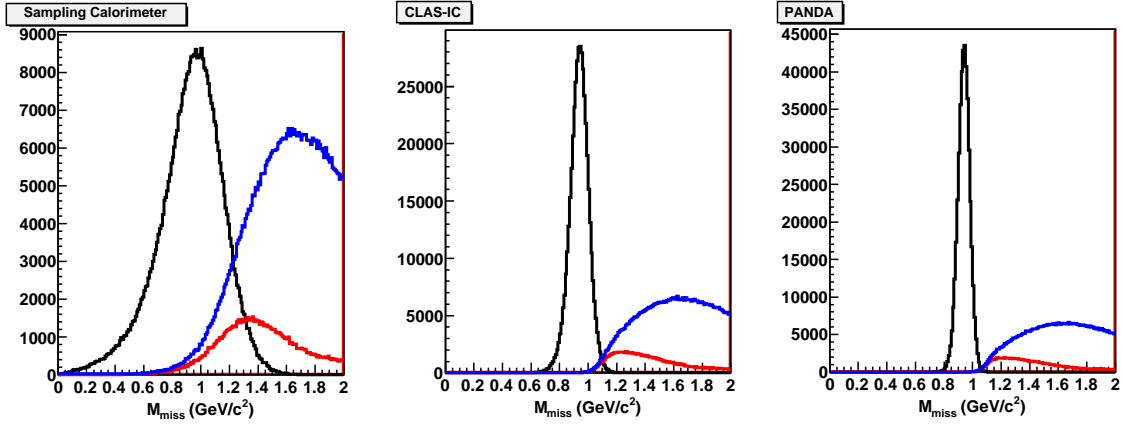
Figure 22: Missing mass of the detected 3\pi system for generated 3\pi events in black, generated 4\pi events with 3 charged \pi detected, in blue and in red the same but with an additional cut on zero \pi^0 decay photons detected. The left plot is for the sampling calorimeter model, middle, the CLAS-IC and right the expected PANDA calorimeter energy resolution.
