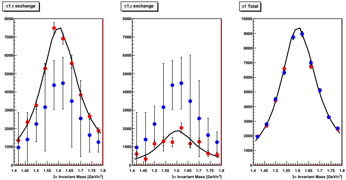
Figure 36: The fit results for the pion exchange mechanism (left), \rho exchange (middle) and total (right). The black line is the generated intensities, while the red circles show the polarized fit and blue, the unpolarized. The large error bars shown in the unpolarized fits are an artifact created by the fitting procedure.
