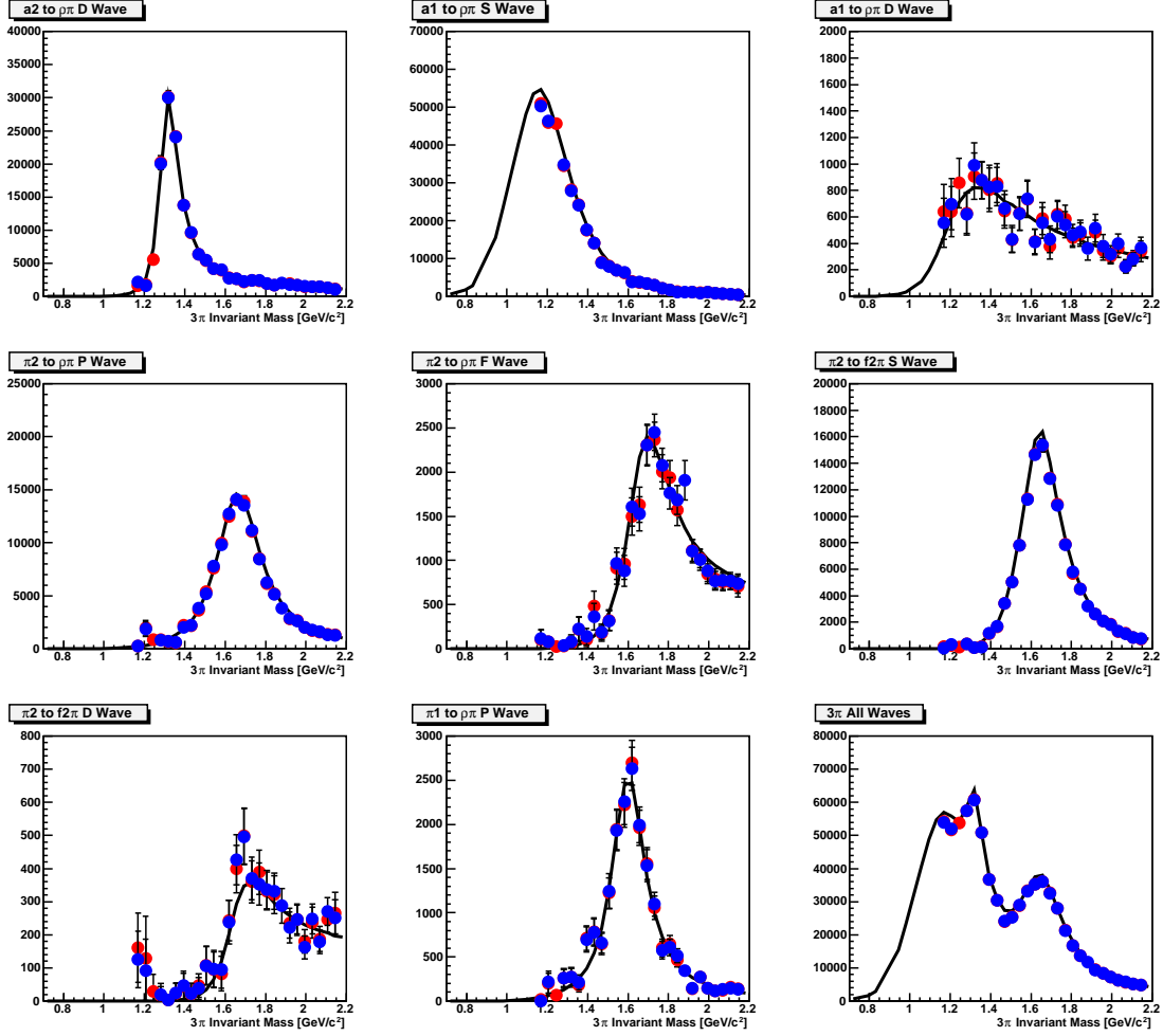
Figure 32: The intensities of the 8 different isobar channels in the 3\pi model, see table 5. The bottom right plot shows the total intensity. The black line shows the generated waves, while the red points are the fit results for t = 0.5(\text{GeV}/c)^2 , half field and the blue points are for “data” tracked resolutions 20% greater than standard, while the corresponding “mc” used standard resolutions.
