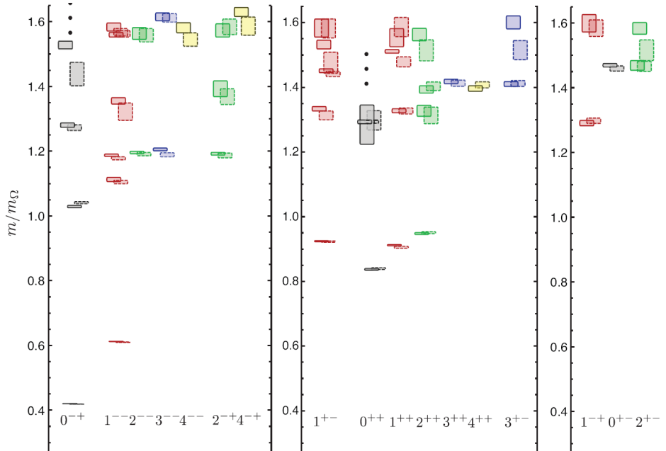
Figure 1: Lattice results from JLab lattice collaboration [9] for the low-lying isovector mesons. Masses are given in units of the \Omega^- baryon mass (1.672 GeV).
