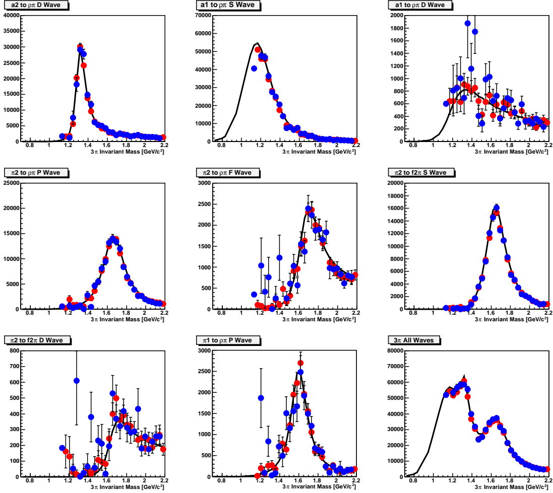
Figure 35: The intensities of the 8 different isobar channels in the 3\pi model, see table 5. The bottom right plot shows the total intensity. The black line shows the generated waves, while the red points are the fit results for t = 0.5(\text{GeV}/c)^2 , half field and the blue points are for full field.
