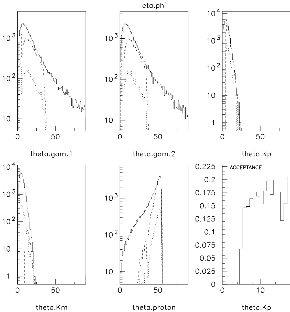
Figure 24: \theta_{Lab} distributions for particles from \phi\eta events and acceptance (bottom right) as a function of the polar angle of the K^+ . The first five panels show the angular distributions for generated (solid) and detected (dashed) particles. In the same panels, the dotted histograms show the angular distributions for events where the final state is identified by detecting the two photons, the K^+ , the proton and reconstructing the K^- with the missing mass technique.
