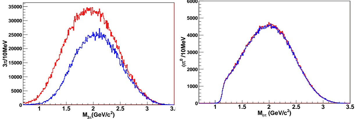
Figure 37: Left: event yield for the reaction \gamma p \rightarrow n\pi^+\pi^+\pi^- as a function of the 3\pi mass for 20 days of beam time at \sim 5 \times 10^{33} \text{cm}^{-2}\text{s}^{-1} luminosity. Right: event yield for the reaction \gamma p \rightarrow p\phi\pi^0 as a function of the \phi\pi mass for 80 days of beam time at 10^{35} \text{cm}^{-2}\text{s}^{-1} luminosity. The red and blue histograms correspond to half and full field configurations of the torus magnet, respectively.
