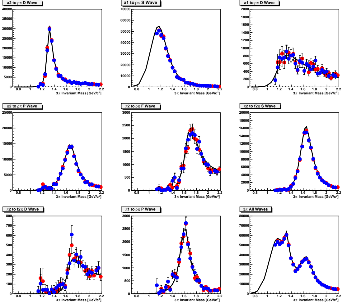
Figure 31: The intensities of the 8 different isobar channels in the 3\pi model, see table 5. The bottom right plot shows the total intensity. The black line shows the generated waves, while the red points are the fit results for t = 0.5(\text{GeV}/c)^2 , half field and the blue points are for “data” tracked with the field incorrectly set 2% higher than for the “mc” events.
