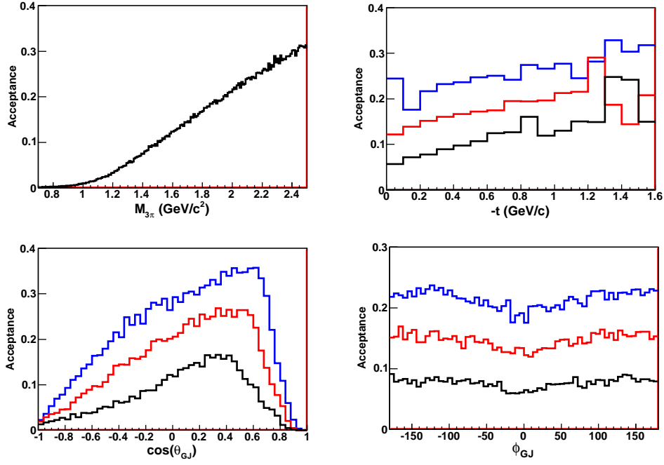
Figure 20: Acceptances for the \pi^+\pi^+\pi^-n final state and half CLAS12 field setting. Top left the 3\pi invariant mass M_{3\pi} , right the momentum transfer t , bottom left, \cos\theta_{GJ} and right, \phi_{GJ} . For the latter 3 plots the black, red and blue lines correspond to M_{3\pi} = 1.4, 1.7 and 2.0 ( \text{GeV}/c^2 ) respectively.
