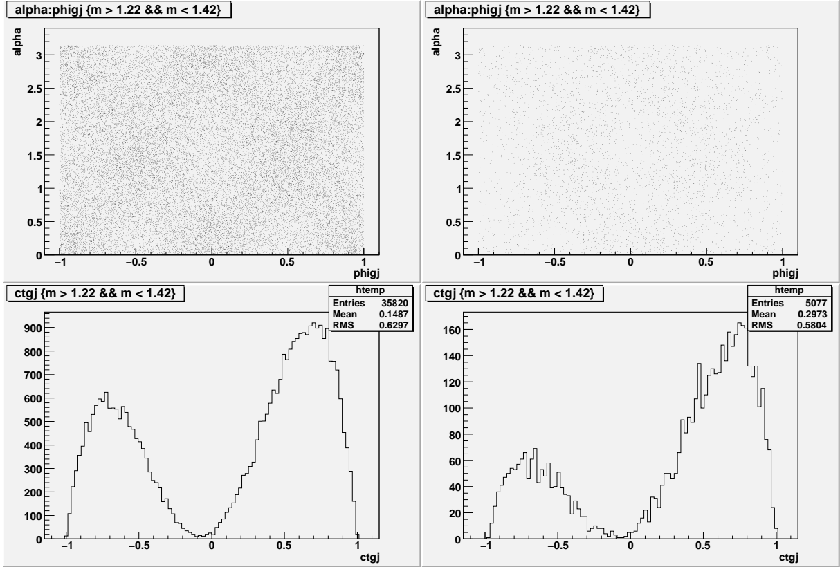
Figure 27: The raw (left) and accepted (right) \phi_{GJ} vs \alpha and \cos(\theta_{GJ}) distributions for the \eta\pi final state.
