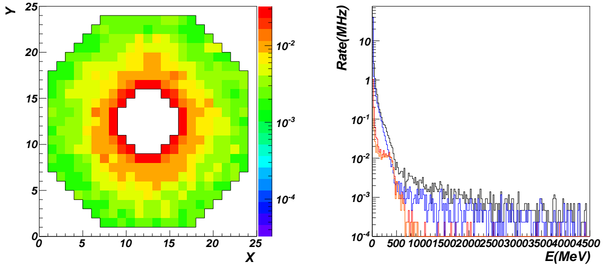
Figure 12: Simulation of the electromagnetic background with GEMC. Left: energy deposited in the calorimeter in MeV/ns. Right: energy distribution of particles hitting the calorimeter front face (black-total, red-electrons, blue-photons).
