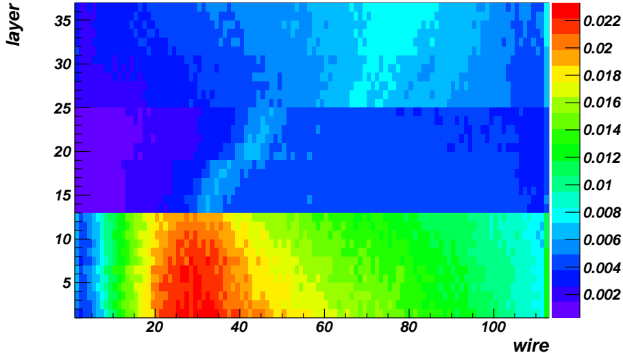
Figure 15: Drift Chamber occupancies at 10^{35} \text{ cm}^{-2}\text{s}^{-1} luminosity as a function of wire and layer number. The maximum occupancy value of about 2% is found in Region 1 while occupancies in Region 2 and 3 are less than 1%. These values are comparable to what estimated in the standard CLAS12 configuration without the FT and are within acceptable values.
