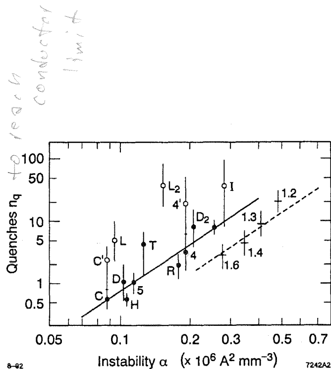
Figure 2. Plot of the number of training quenches versus the instability factor \alpha , as defined in the text, for magnets from : (T) Tevatron; (H) HERA; (C) CBA; (D) DESY; (I) Isabelle; (R) RHIC; (4) SSC, 4 cm; (5) SSC, 5 cm; (Q) SSC, quads; (L) LHC; 1.2, 1.3, 1.4, 1.6 SSC cables with those Cu/sc ratios. When primed, the data refer to early prototypes or magnets with problems. When given a subscript of 2, the data refer to tests at 1.8^\circ .
