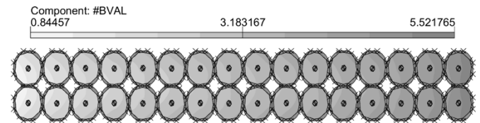
Fig. 4. Magnetic field distribution in the Rutherford cable, when an external field of 3.18 T is applied.
