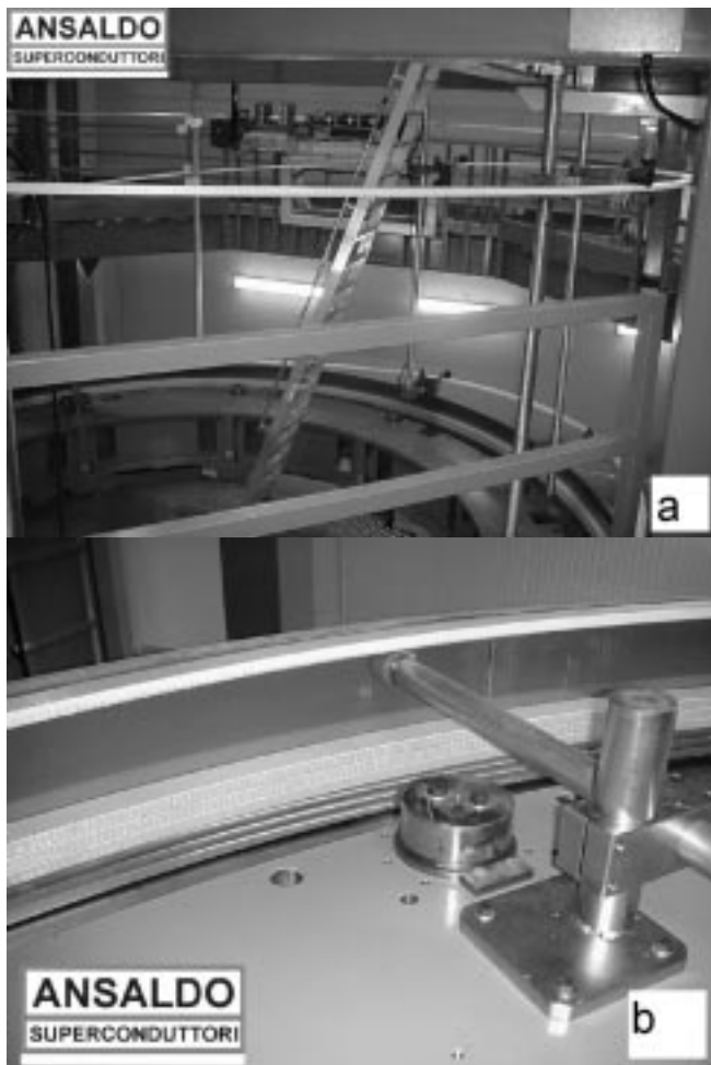
Fig. 10. Dummy conductor after (a) bending and (b) transferring.
