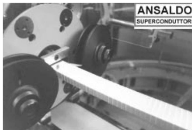
Fig. 7. Taping unit mounted in the winding line.
