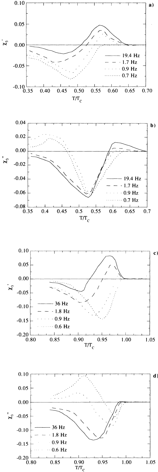
FIG. 5. Third harmonics of the BISCCO1 sample (a) in-phase; (b) out-of-phase with T_c(B=1 \text{ T}) = 85 \text{ K} , and for the NTTZ1 sample (c) in-phase; (d) out-of-phase with T_c(B=1 \text{ T}) = 8.55 \text{ K} . To be noted that in the Bi-based sample the onset of harmonics is the irreversibility temperature T_{irr}=0.7T_c=59.5 \text{ K} .
