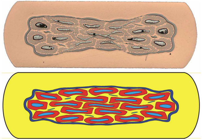
Fig. 5. ALSTOM/CEA \text{Nb}_3\text{Sn} internal tin wire after a 48% reduction in diameter. The observed deformation is shown together with the FE analysis result.
