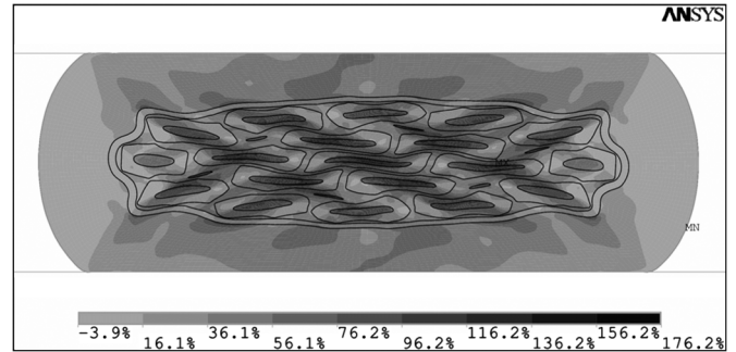
Fig. 6. Total strain in the x direction of the ALSTOM/CEA \text{Nb}_3\text{Sn} internal tin wire after a 48% reduction in diameter.
