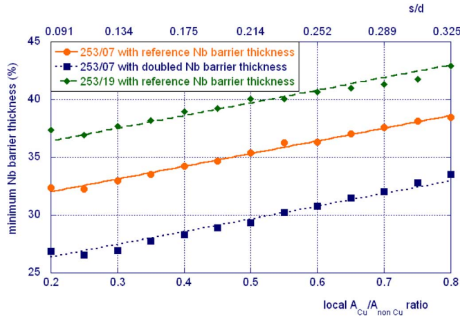
Fig. 8. Minimum thickness of Nb barrier with respect to its nominal value after 28% reduction in diameter of the wire as function of the local-Cu-to-non-Cu ratio for the 253/07 configuration with reference ( 2.2 \mu\text{m} ) and double ( 4.4 \mu\text{m} ) Nb barrier thickness and for the 253/19 configuration with reference Nb barrier thickness ( 2.2 \mu\text{m} ). For completeness, the s/d values (spacing between sub-elements over sub-elements diameter) are also shown.
