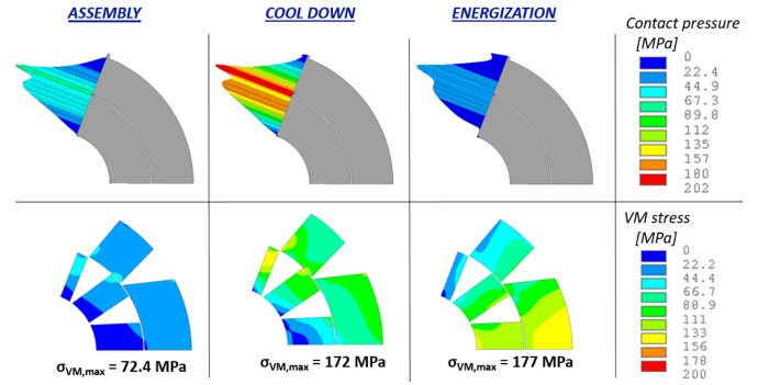
Fig. 5. FE analysis results at the nominal field of 14 T: in the first line the pole-coil contact pressure plot and in the second one the VM stresses in the coils, computed in the three simulation steps.
