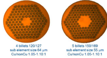
Fig. 5. Conductors for the first ERM and RMM coils, Bruker-OST.
