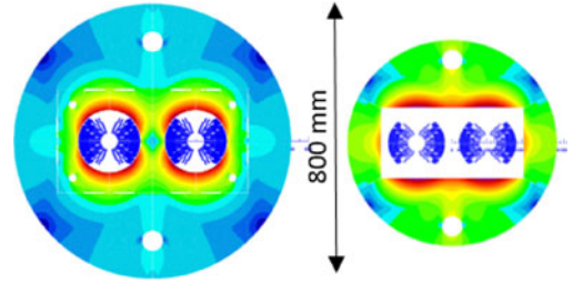
Fig. 1. \cos\theta : electromagnetic cross section (left 2015, right 2017).
