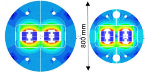
Fig. 2. Block-coil: electromagnetic cross section (left 2015, right 2017).
