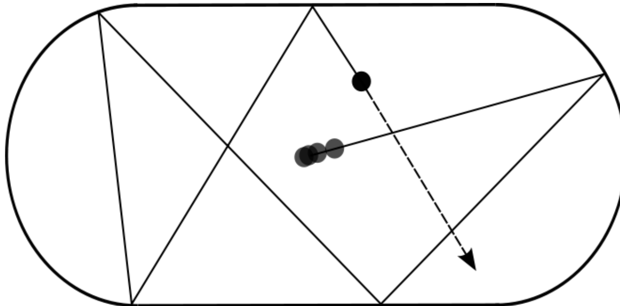
The Bunimovich stadium. Proof of ergodicity 1979.
