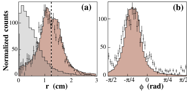
FIG. 3 (color). (a) Comparison of radial ( r ) annihilation distributions ( dN/drdr ) for the data from the low pressure measurement (error bars) and the MC simulations assuming annihilations on the trap wall (brown histogram). The inner radius of the trap electrodes is indicated with a dashed line. Also shown are the data for the high pressure measurement (grey histogram). (b) The azimuthal ( \phi ) angular distribution of the annihilation (error bars) and its comparison with the MC assuming point source annihilation.
