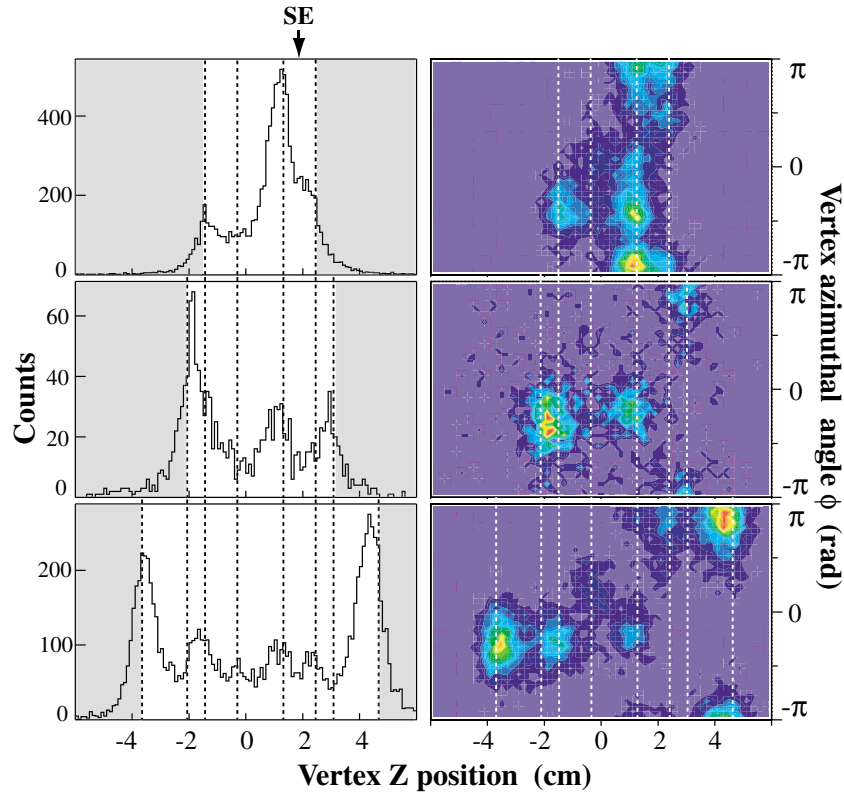
FIG. 5 (color). Similar to Fig. 4, but with varying numbers of electrodes used in the trap well, shown as unshaded regions. “SE” indicates the fourfold azimuthally sector electrode.
