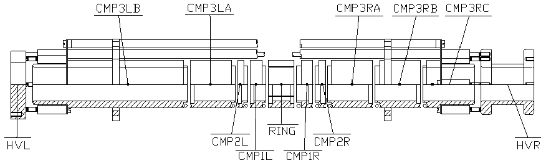
FIGURE 1. Configuration of the antiproton catching trap electrodes
