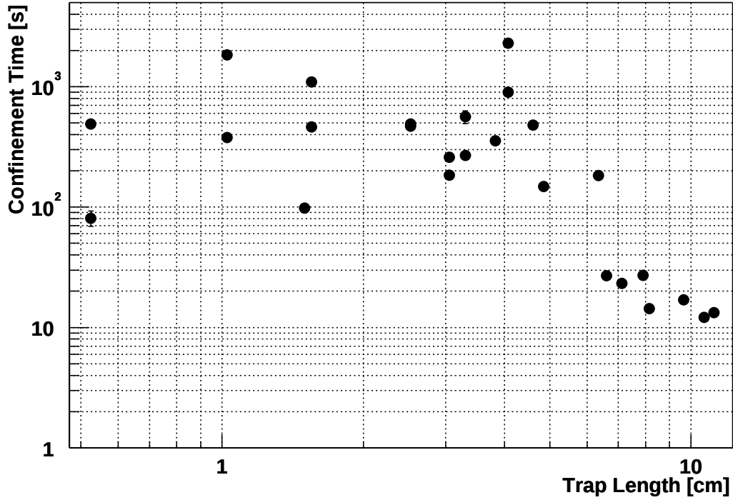
FIGURE 3. Dependence of confinement time on trap length. The confinement time is defined like the required time for one-half of the injected electrons to be lost.
