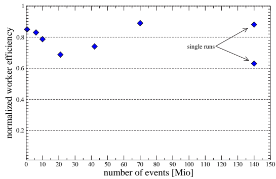
Figure 3: Normalized, average worker efficiency for large Geant 4 simulation using explicit worker placement with ssh. Interactive cluster.
