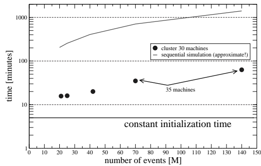
Figure 2: Average execution times for large Geant 4 simulation using explicit worker placement with ssh. Interactive cluster.
