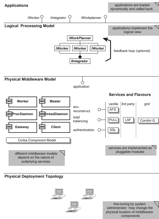
Figure 1: Overview of DIANE's layered architecture.
