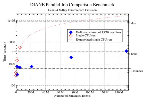
Figure 4: Average execution times for large Geant 4 simulation using explicit worker placement with ssh. Dedicated cluster.
