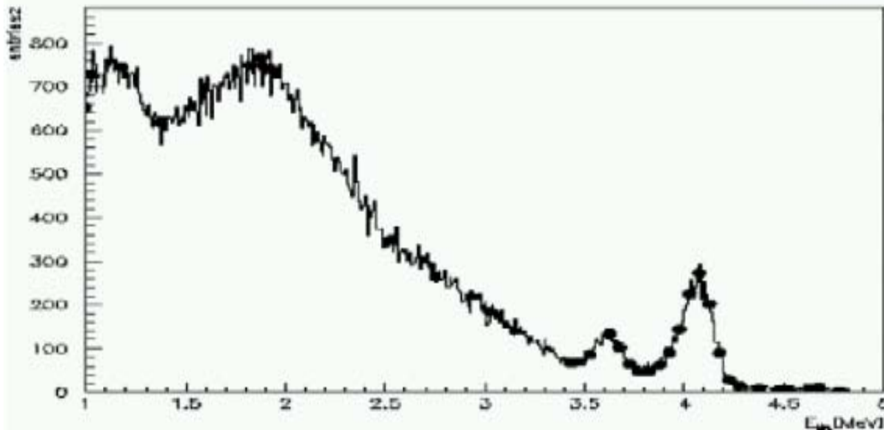
Geant4 simulation of gammas from 14 MeV neutron capture on uranium.
