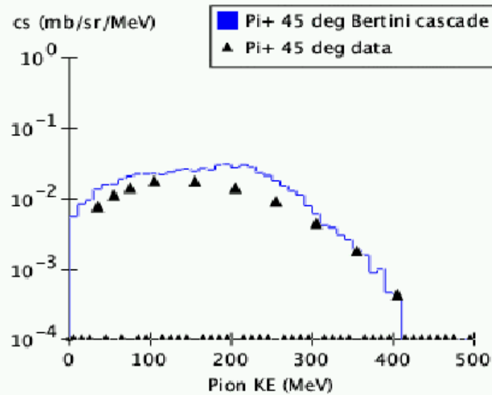
730 MeV p on C
