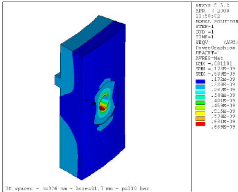
Fig. 3 : FEA analysis of the titanium spacer.
