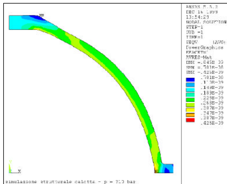
Fig. 4 : FEA analysis of the spherical caps.
