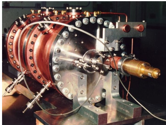
RF Separators
