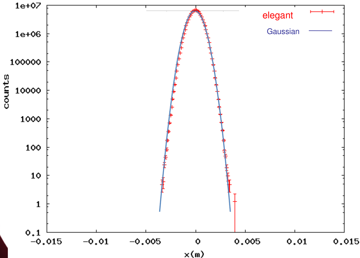
X profile at hallID radiator
