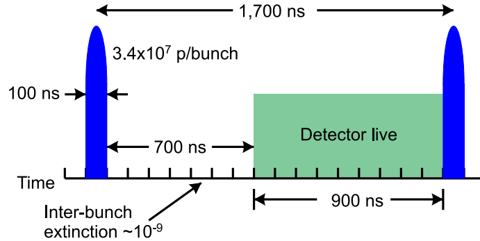
Figure 2.3: The proton beam bunch scheme. Every 1.7 \mu s a bunch of 3.4 \times 10^7 protons is delivered to the muon production target. For 700 ns after the end of the 100 ns wide bunch the detector is off.
