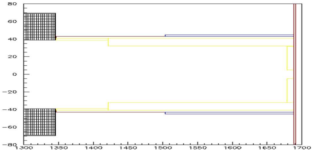
Figure 8.7: Beam stop design showing CH 2 (yellow), stainless steel (red), Lead (blue), and the calorimeter (black cross-hatched).
