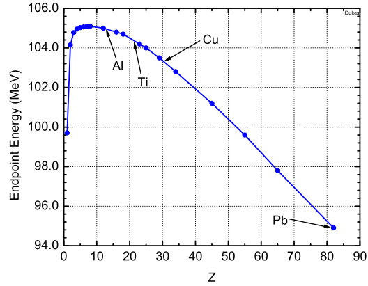
Figure 10.2: The stopped muon lifetime vs Z . Figure 10.3: The muon decay-in-orbit endpoint energy vs Z .
