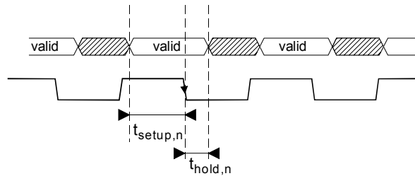
Figure 5 Definition of data setup and hold times for the case that the falling edge of clkLHC is used to validate the data ( conf_negedge = 1).
