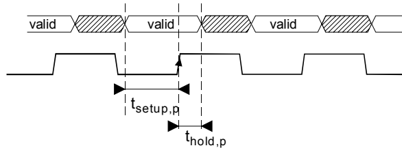
Figure 4 Definition of data setup and hold times for the case that the rising edge of clkLHC is used to validate the data ( conf_negedge = 0).
