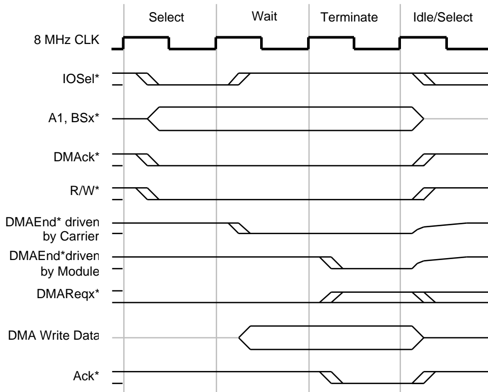
Figure 9 8 MHz DMA Write Cycle with Wait State
