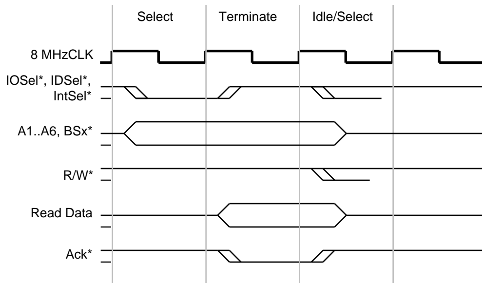
Figure 3 Fastest 8 MHz Read Cycles
