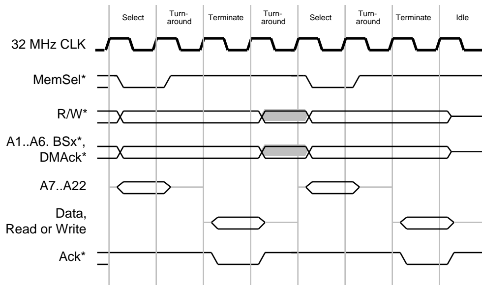
Figure 18 32 MHz Two Memory Cycles Back to Back
