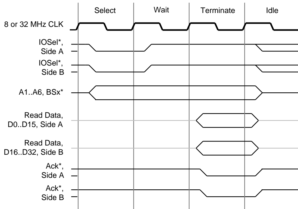
Figure 10 32-bit Double-size Operation
