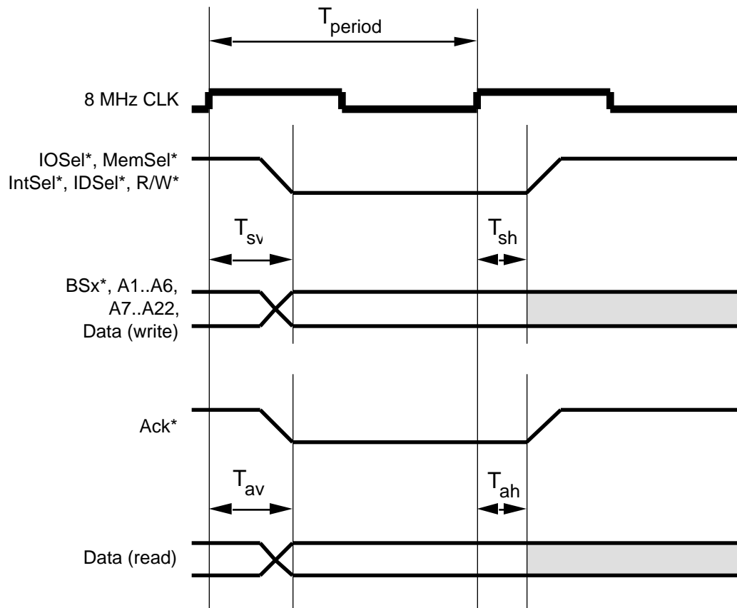
Figure 12 8 MHz Detailed Timing Diagram
