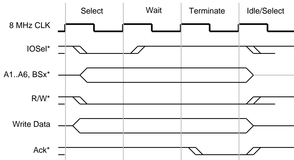
Figure 6 8 MHz I/O Write Cycle with Wait State
