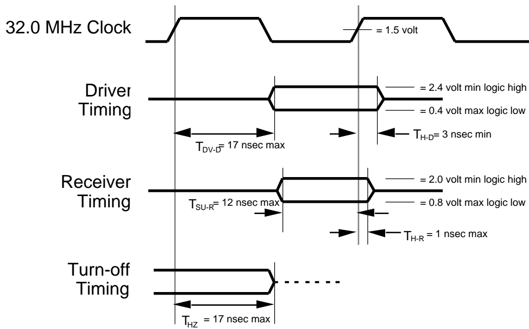
Figure 22 32 MHz Detailed Timing
