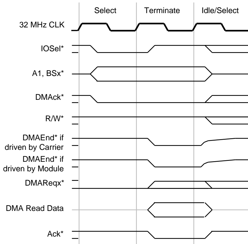
Figure 20 32 MHz DMA I/O Read Cycle
