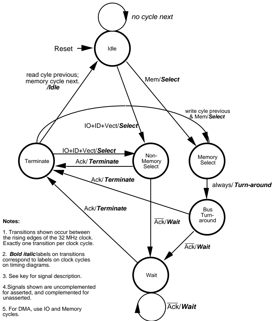
Figure 21 32 MHz State Diagram
