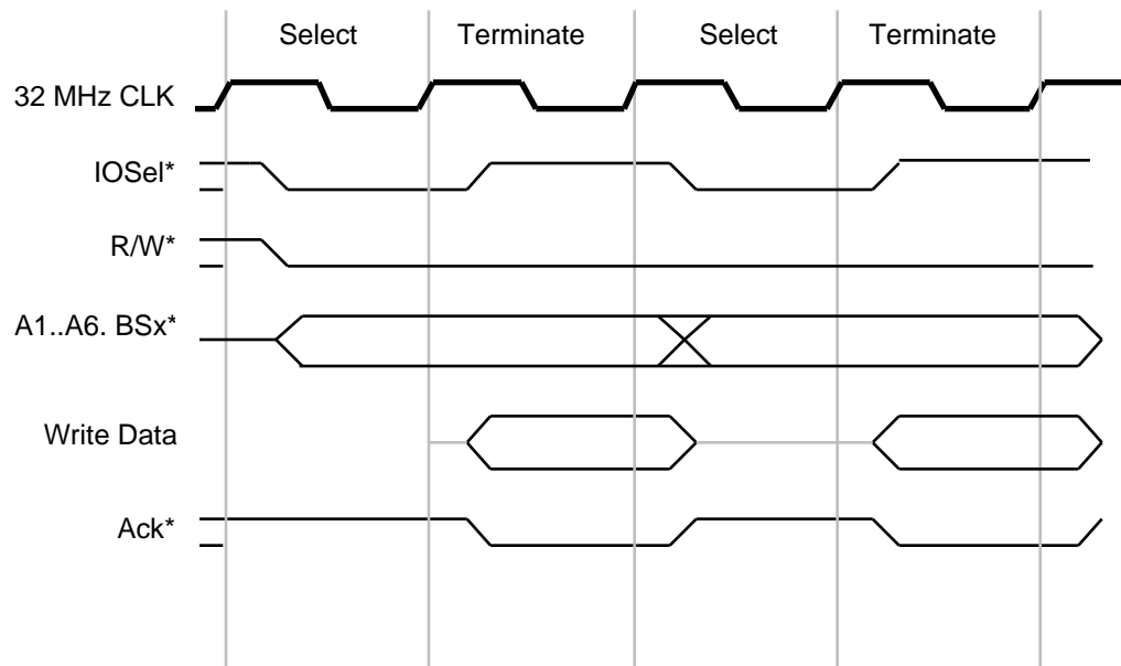
Figure 13 32 MHz Two I/O Write Cycles Back to Back
