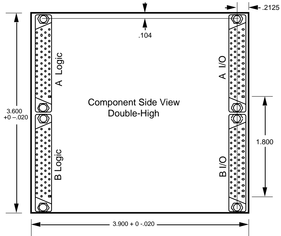
Figure 26 Double-size Module Mechanical
