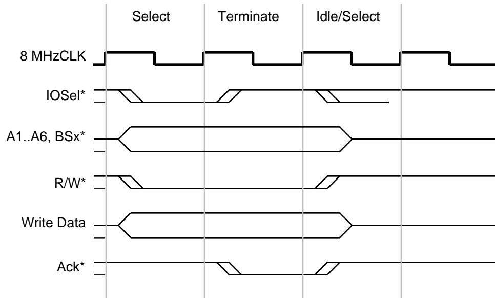
Figure 2 Fastest 8 MHz I/O Write Cycle
