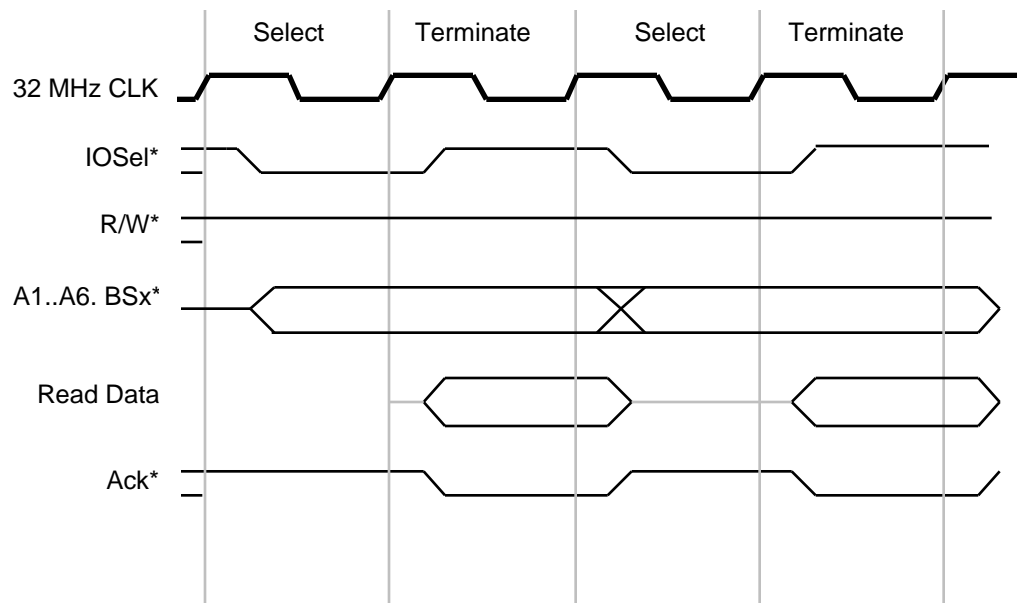
Figure 14 32 MHz Two I/O Read Cycles Back to Back
