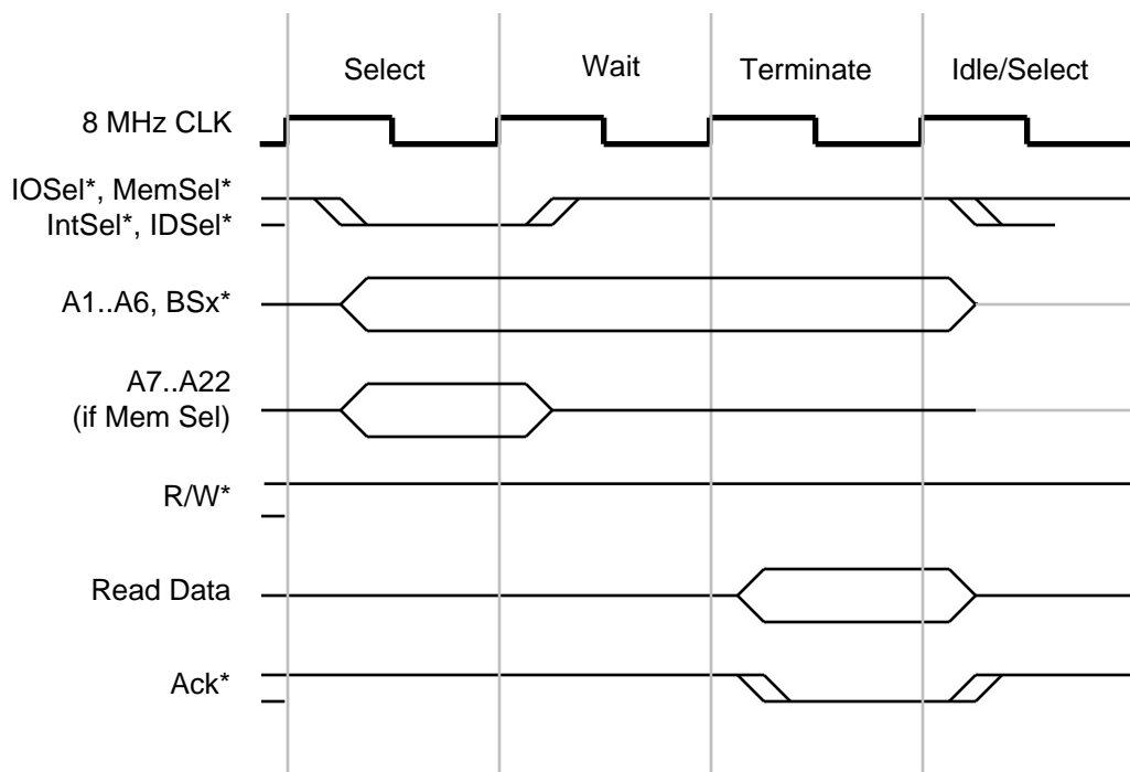
Figure 5 8 MHz Read Cycle with Wait State
