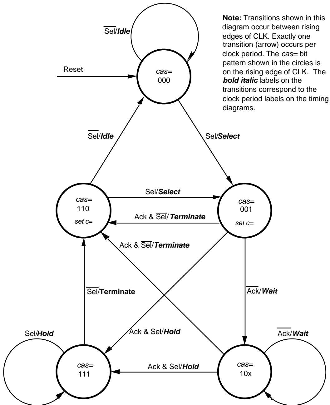
Figure 11 8 MHz State Diagram
