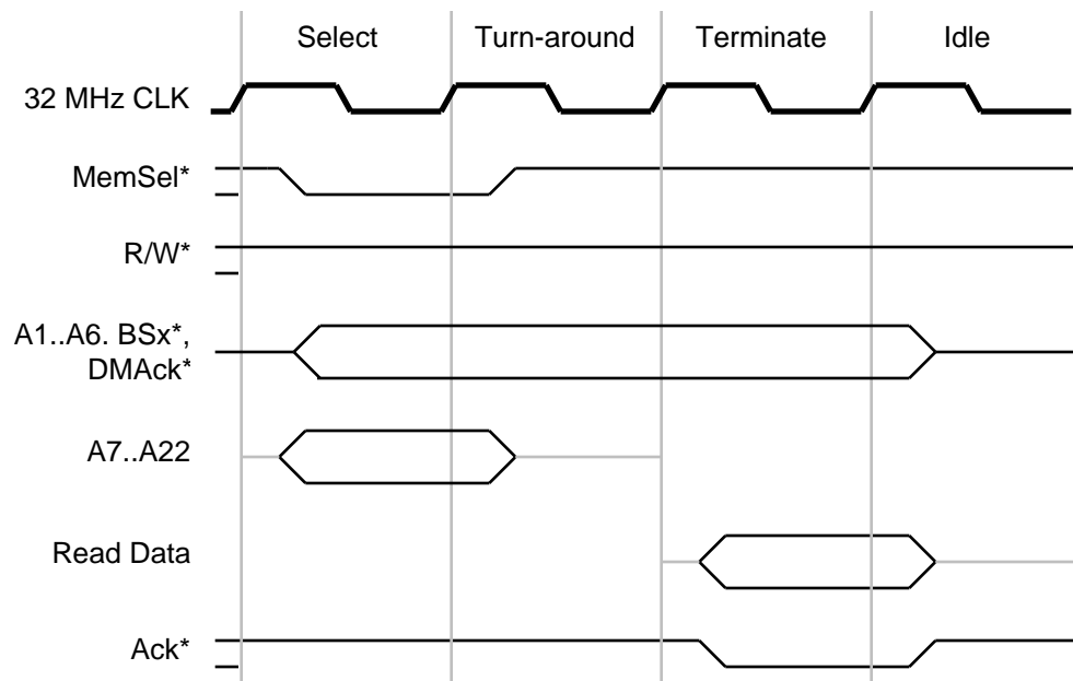
Figure 16 32 MHz Fastest Memory Read Cycle
