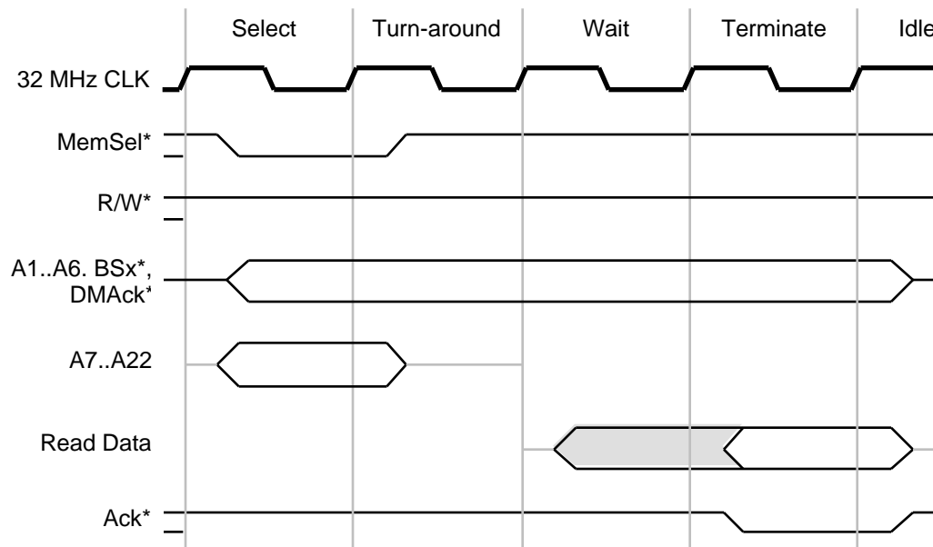
Figure 17 32 MHz Memory Read Cycle with Wait State
