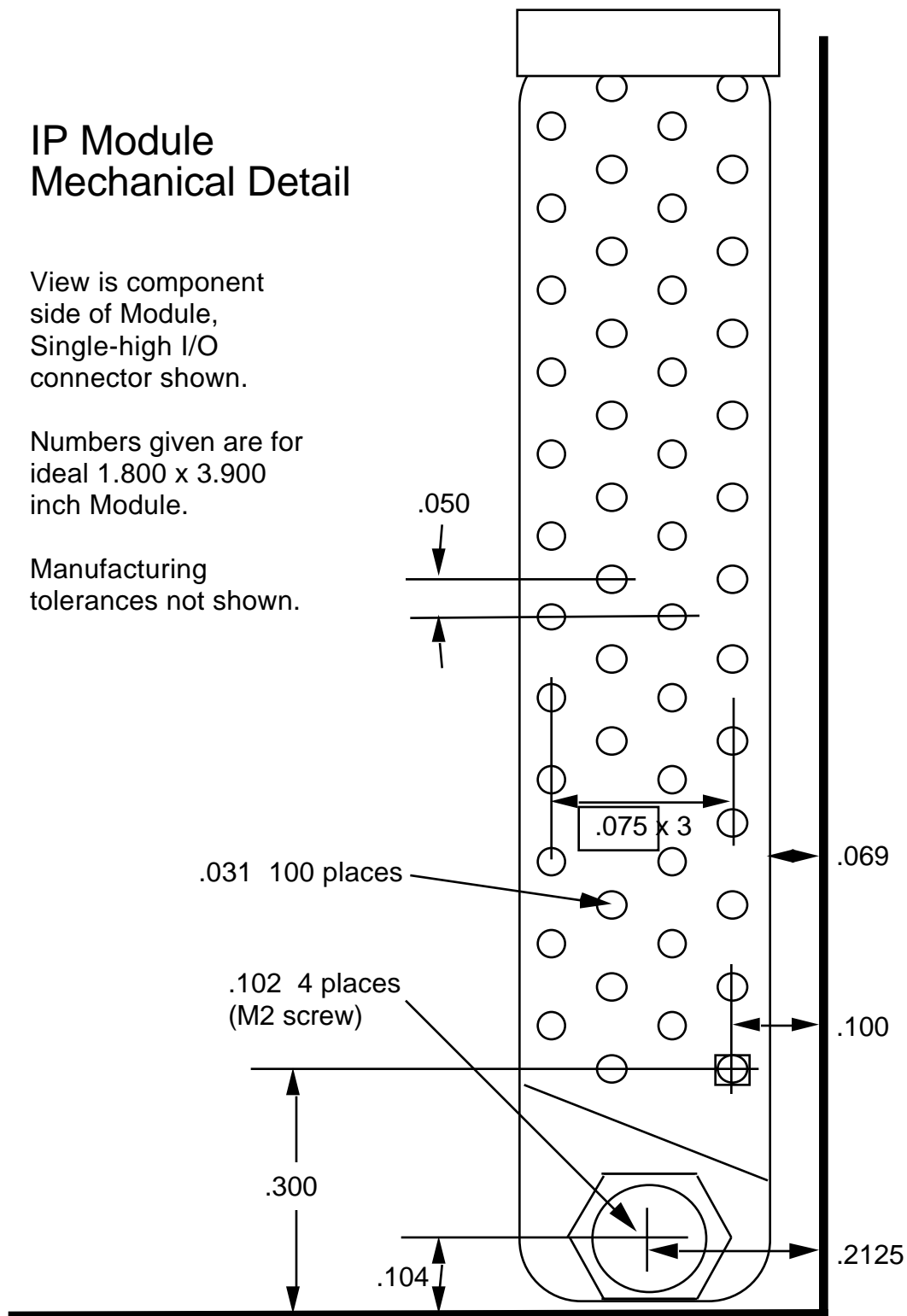
Figure 24 IP Module Mechanical Detail
