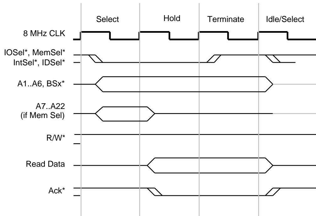
Figure 4 8 MHz Read Cycle with Hold State
