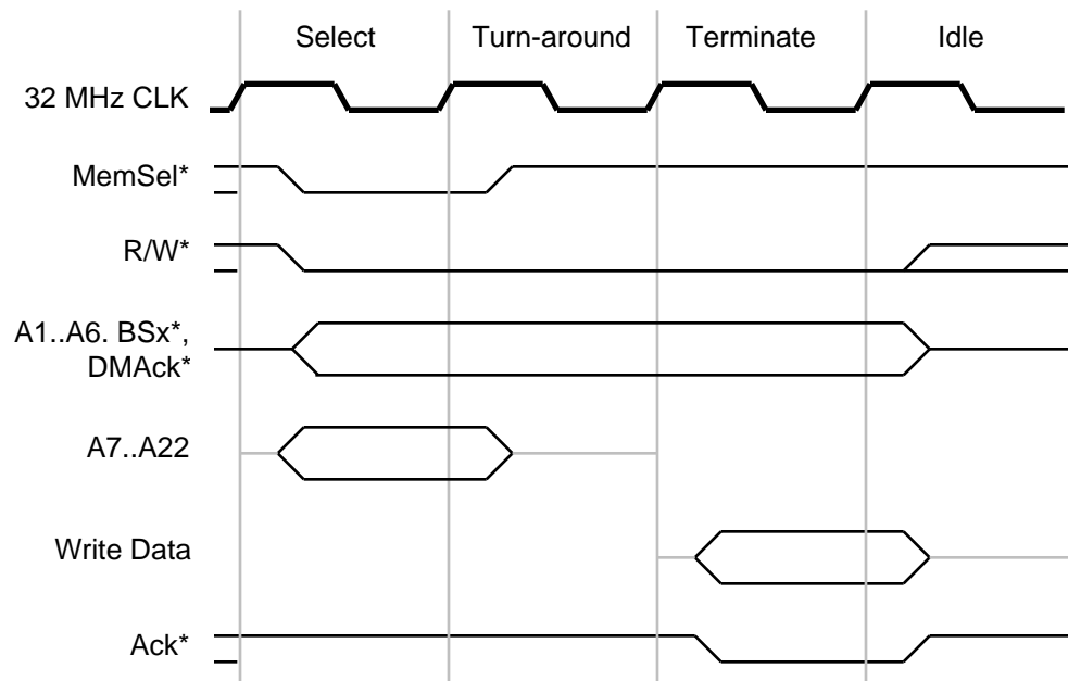
Figure 15 32 MHz Fastest Memory Write Cycle
