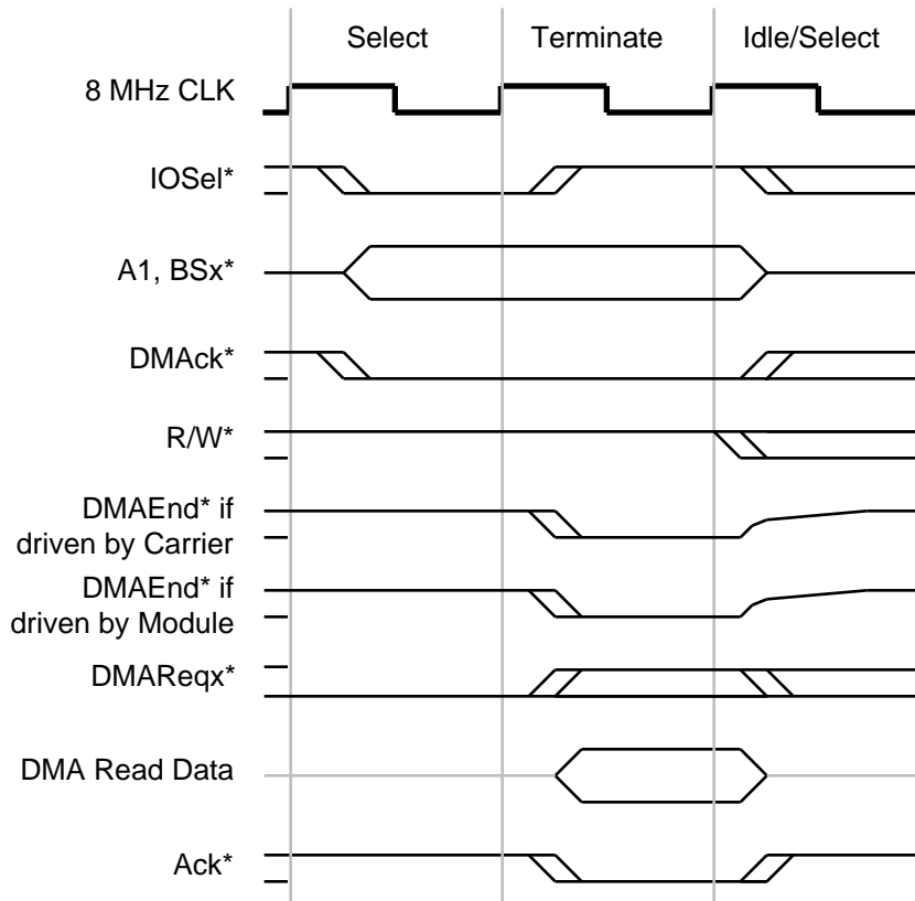
Figure 8 8 MHz DMA Read Cycle
