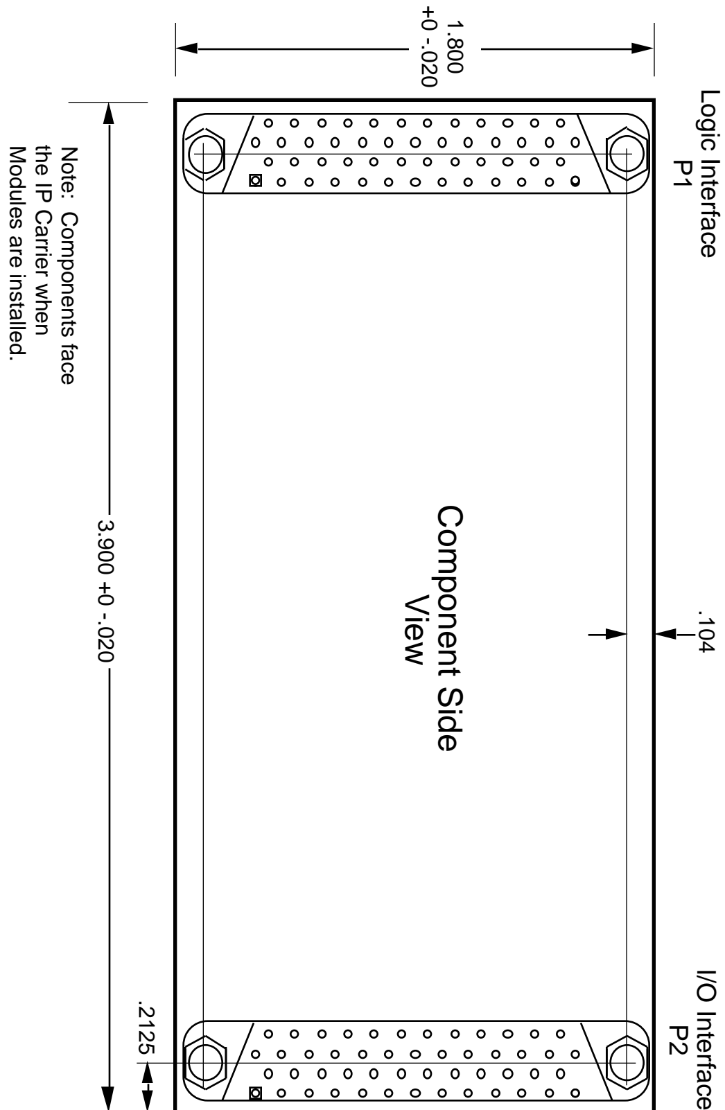
Figure 23 Single-size IP Module Mechanical Outline
