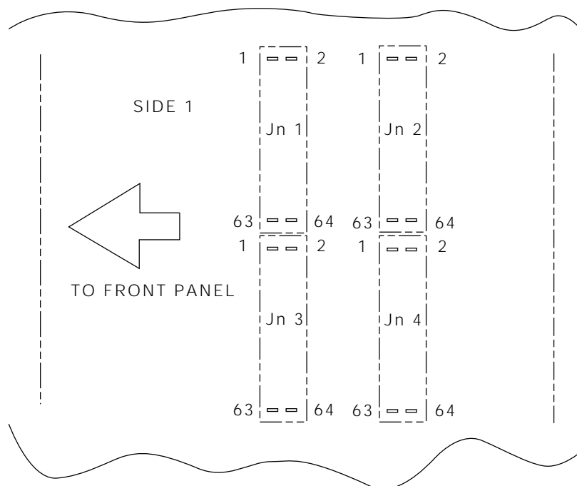
Figure 5-2 Connector Orientation on Host, Side 1
