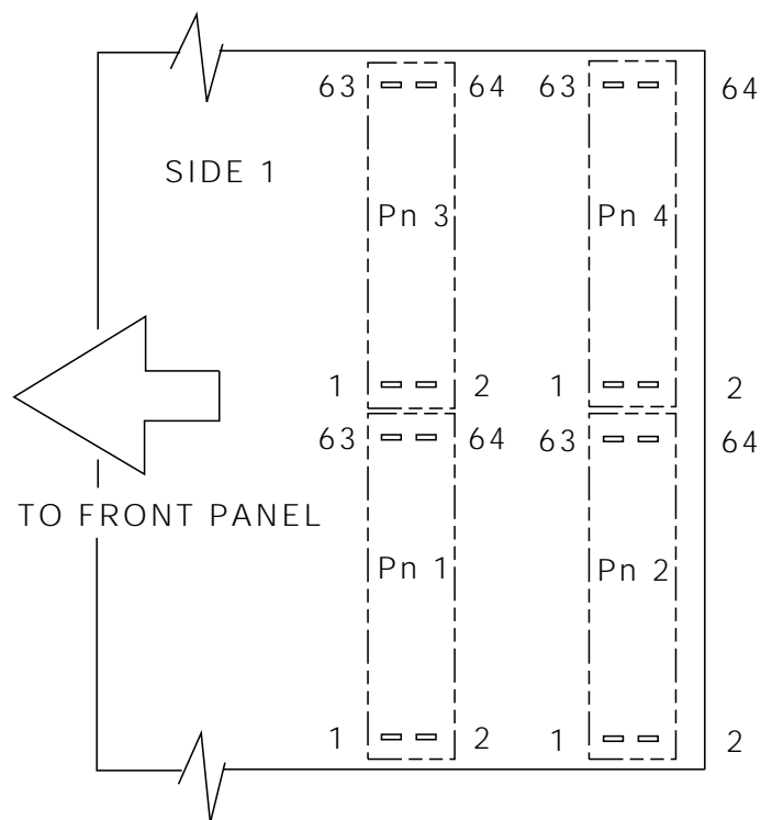
Figure 5-1 Connector Orientation on PMC, Side 1
