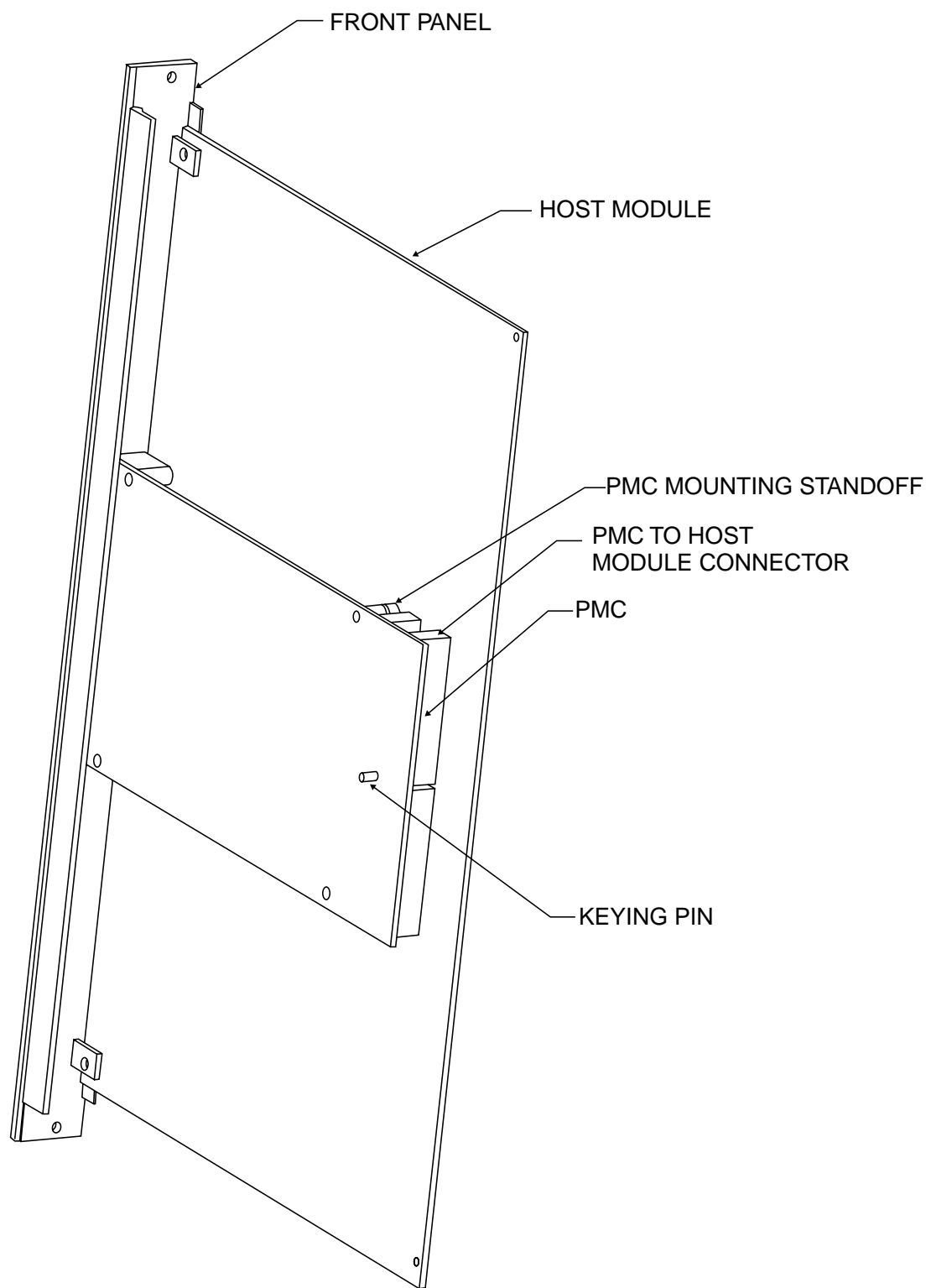
Figure 1-1 Typical PMC Mounted to a Host Module
