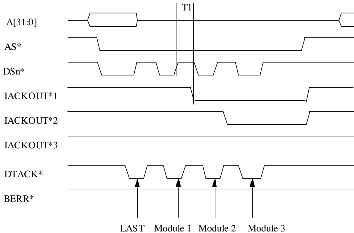
Figure E.8-2 D64 CBLT Slave Responses
