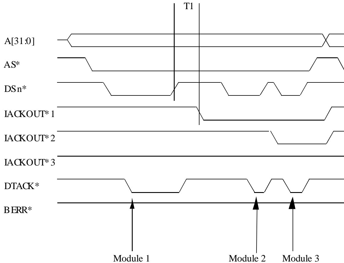
Figure E.8-1 D32 CBLT Timing, Slave Responses
