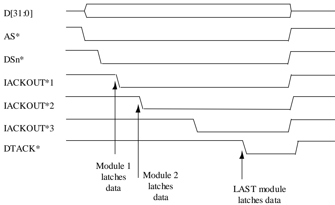
Figure E.8-4 MCST Timing
