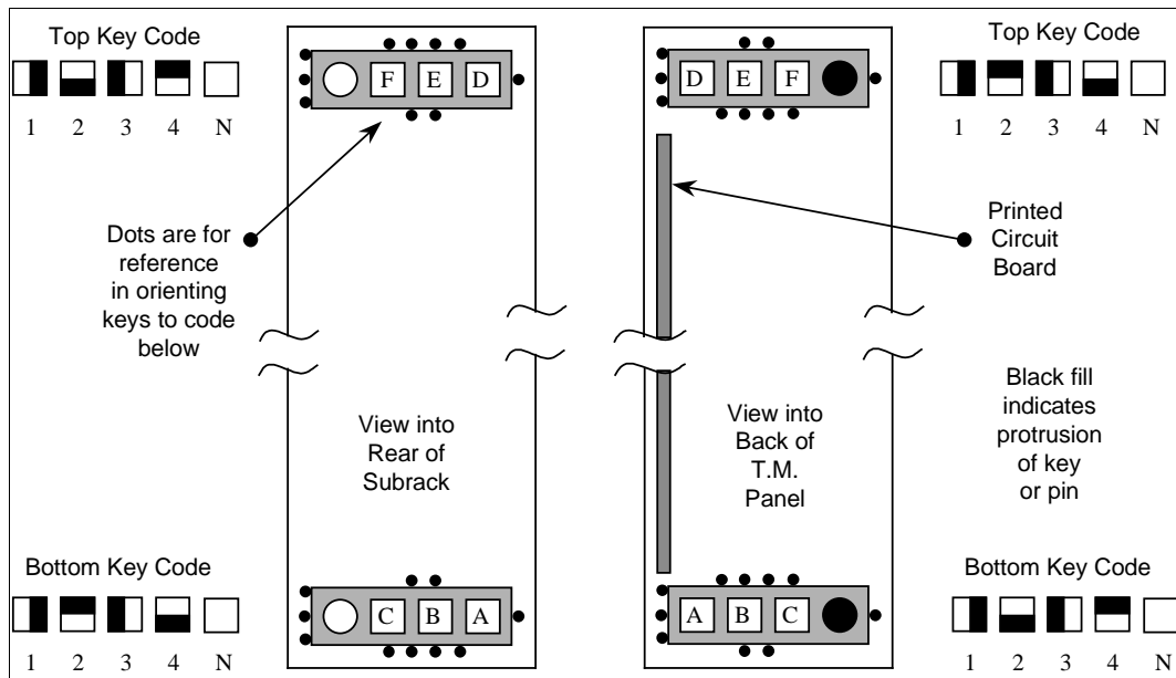
Figure C.4-2 Transition Module Keying Hole Positions and Associated Keying Codes
