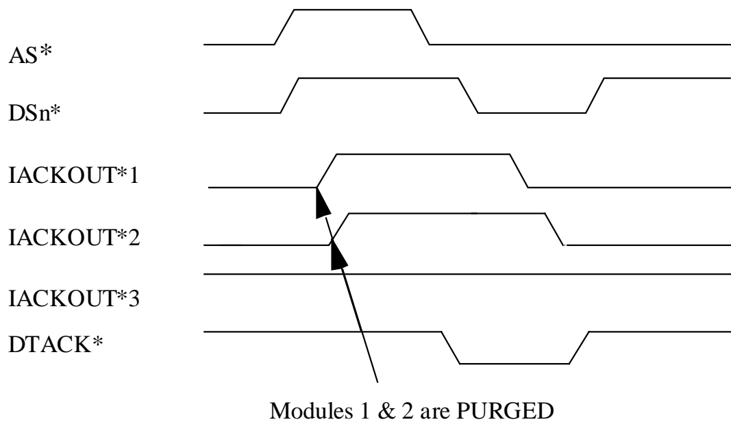
Figure E.8-3 Multiple CBLT Timing Short Cut
