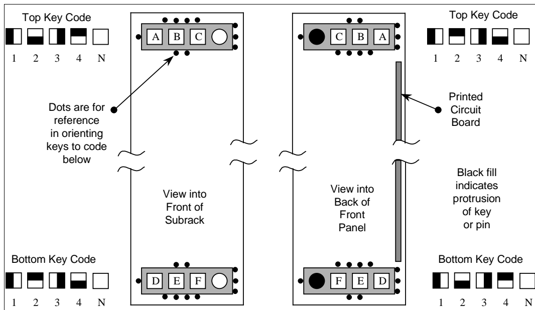
Figure C.4-1 VME Module Keying Hole Positions and Associated Keying Codes
