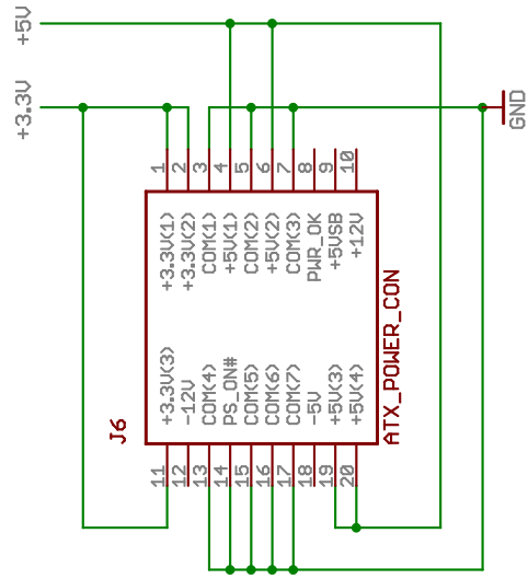
ATX Power Supply Connector
